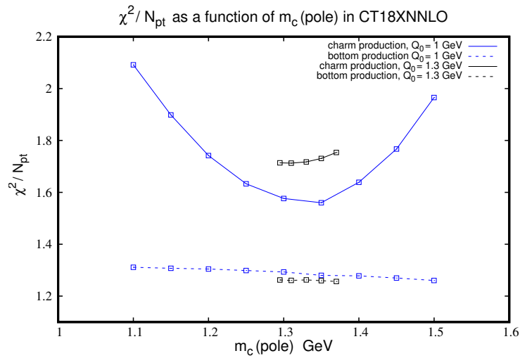
Figure 1: \chi^2/N_{pt} for charm (solid) and bottom (dashed) production in the CT18XNNLO fit as a function of the charm-quark mass m_c(\text{pole}) for different values of the input scale Q_0 .
