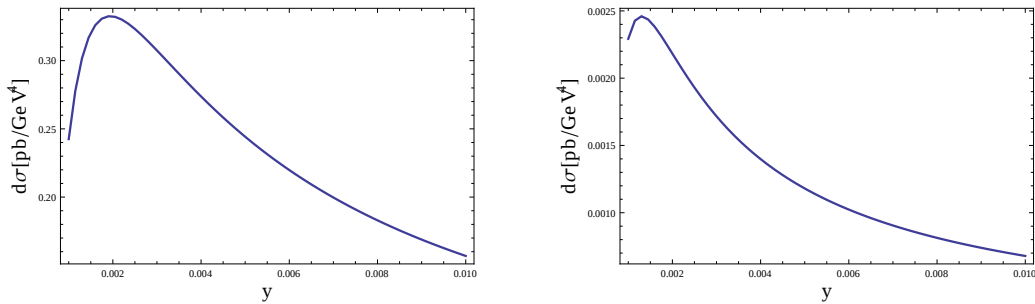
Figure 4: Left panel : The y dependence of the longitudinal cross section \frac{d\sigma(e^-N \rightarrow \nu ND_s^{*-})}{dy dQ^2 dt} (in pb \text{GeV}^{-4} ) for \Delta_T = 0 and s = 20000 \text{ GeV}^2 and Q^2 = .1 \text{ GeV}^2 . Right panel : idem for the production cross-section of a transversely polarized D_s^{*-} .
