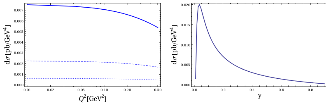
Figure 2: Left panel : The Q^2 dependence of the cross section \frac{d\sigma(e^-N \rightarrow \nu ND_s^-)}{dy dQ^2 dt} (in \text{pb GeV}^{-4} ) for \Delta_T = 0 and s = 820 \text{ GeV}^2 and y = .2 (solid curve) , y = .5 (dashed curve) and y = .8 (dotted curve). Right panel : The y dependence of the cross section \frac{d\sigma(e^-N \rightarrow \nu ND_s^-)}{dy dQ^2 dt} (in \text{pb GeV}^{-4} ) for Q^2 = 0.1 \text{ GeV}^2 , \Delta_T = 0 and s = 820 \text{ GeV}^2 .
