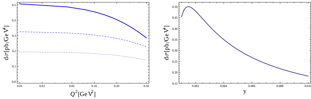
Figure 3: Left panel : The Q^2 dependence of the cross section \frac{d\sigma(e^-N \rightarrow \nu ND_s^-)}{dy dQ^2 dt} (in pb \text{GeV}^{-4} ) for \Delta_T = 0 and s = 20000 \text{ GeV}^2 and y = 10^{-3} (solid curve) , y = 5 \cdot 10^{-3} (dashed curve) and y = 10^{-2} (dotted curve). Right panel : The y dependence of the cross section \frac{d\sigma(e^-N \rightarrow \nu ND_s^-)}{dy dQ^2 dt} (in pb \text{GeV}^{-4} ) for Q^2 = 0.1 \text{ GeV}^2 , \Delta_T = 0 and s = 20000 \text{ GeV}^2 .
