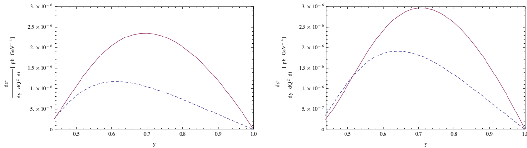
Figure 1: The y dependence of the longitudinal contribution to the cross section \frac{d\sigma(\nu N \rightarrow l^- ND^+)}{dy dQ^2 dt} (in \text{pb GeV}^{-4} ) for Q^2 = 1 \text{ GeV}^2 , \Delta_T = 0 and s = 20 \text{ GeV}^2 for a proton (left panel) and neutron (right panel) target : total (quark and gluon, solid curve) and quark only (dashed curve) contributions.
