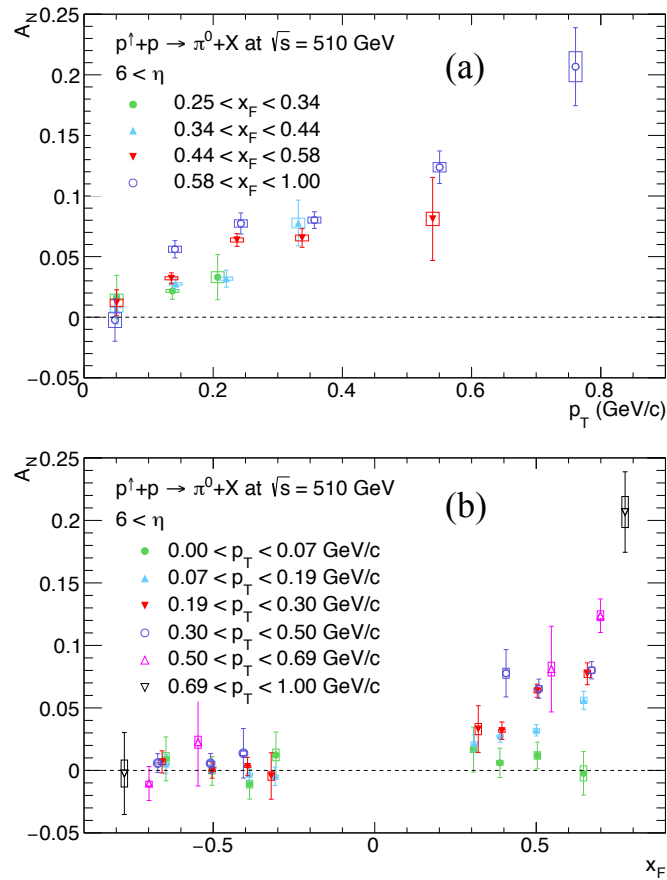
Figure 3: A_N of the very forward \pi^0 s as functions of (a) p_T for several x_F ranges and (b) x_F for several p_T ranges. Only forward A_N was presented in (a). Error bars represent the statistical uncertainties, and the boxes represent the systematic uncertainties.
