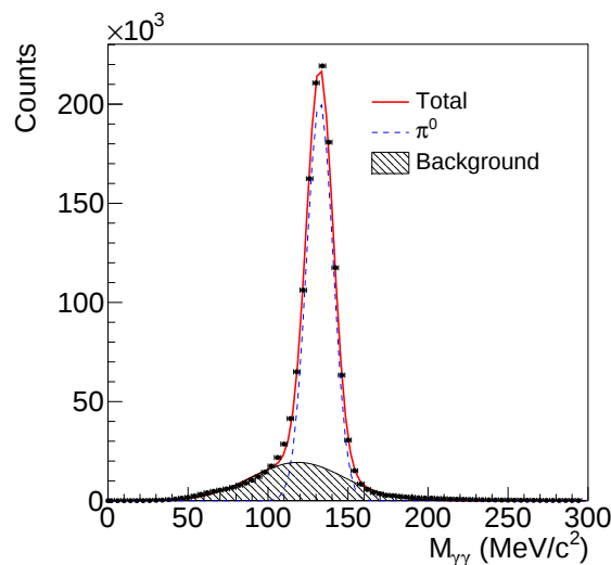
Figure 2: Reconstructed two photon invariant mass distribution of Type-I event in x_F > 0.25 and 0.0 < p_T < 1.0 \text{ GeV}/c .
