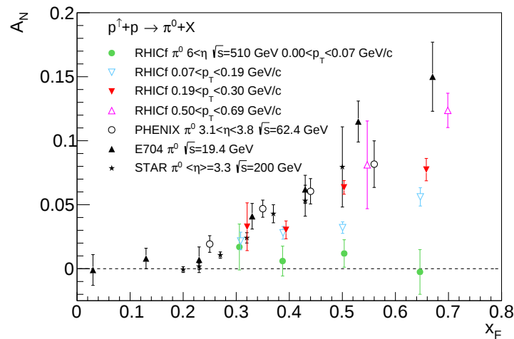
Figure 4: Comparison of the RHICf data with the previously measured A_N of the forward \pi^0 s as a function of x_F .
