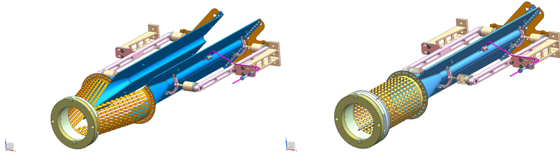
Figure 1: SMOG2 storage cell in open (left) and closed (right) configuration.
