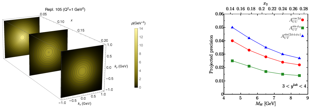
Figure 3: Left: up quark densities in momentum space [12]. Right: projected precision for some TSSAs with Drell-Yan data [7] with x_2 being the longitudinal momentum fraction of the target nucleon and M_{\ell\ell} the dilepton invariant mass.
