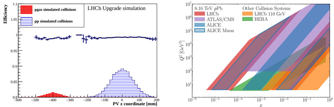
Figure 2: Left: Reconstruction efficiency for beam-gas (red) and beam-beam (blue) primary vertices [6]. Right: kinematic coverage of LHCspin (orange) and other existing facilities.
