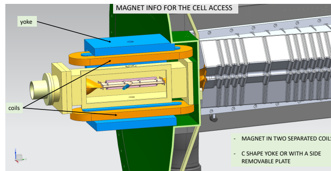
Figure 4: The TC drawing with the magnet coils (orange) and the iron return yoke (blue) enclosing the storage cell. The VELO vessel and detector box are shown in green and grey, respectively.
