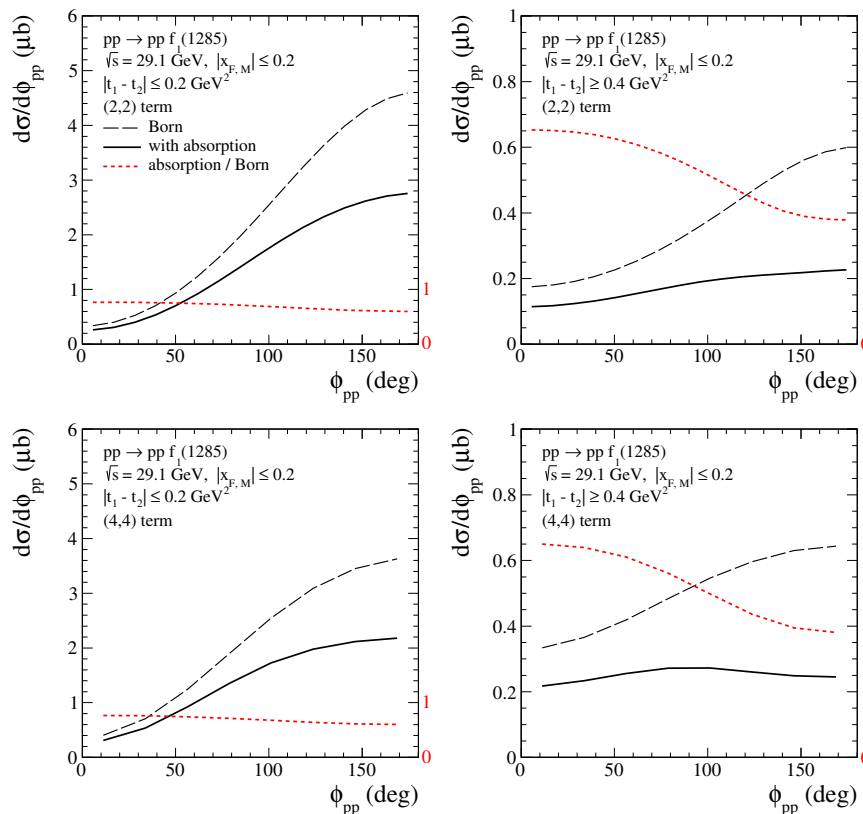
Figure 3: The \phi_{pp} distributions for f_1(1285) meson production at \sqrt{s} = 29.1 \text{ GeV} , |x_{F,M}| \leq 0.2 , for |t_1 - t_2| \leq 0.2 \text{ GeV}^2 (left) and for |t_1 - t_2| \geq 0.4 \text{ GeV}^2 (right). The long-dashed black lines represent the Born results and the solid black lines correspond to the results with the absorption effects included. The dotted red lines represent the ratio of full and Born cross sections on the scale indicated by the red numbers on the r.h.s. of the panels.
