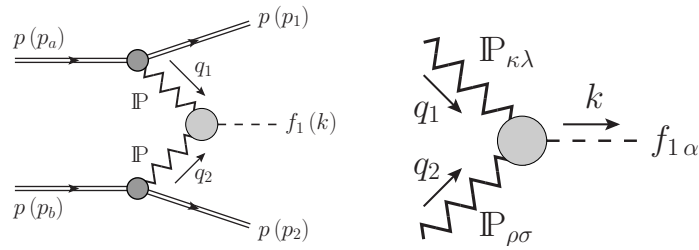
Figure 1: Diagrams for the reaction (1) with double- \mathbb{P} exchange and the \mathbb{P}\mathbb{P}f_1 vertex.
