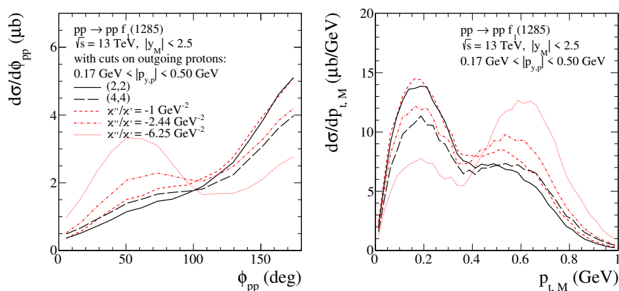
Figure 4: The differential cross sections for the f_1(1285) production at \sqrt{s} = 13 TeV, |y_M| < 2.5 , and with cuts on momenta of outgoing protons ( 0.17 \text{ GeV} < |p_{y,p}| < 0.50 \text{ GeV} ). The results for (l, S) and (\chi', \chi'') terms are shown.
