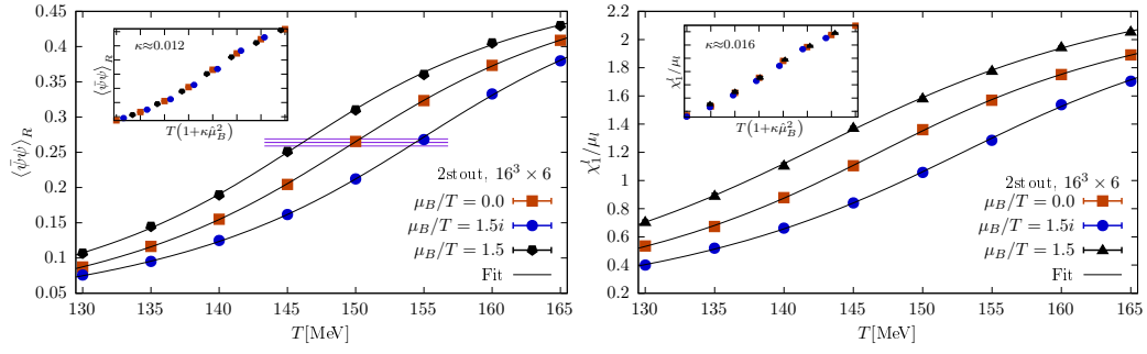
Figure 2: The renormalized chiral condensate (left) and the light quark number-to-light quark chemical potential ratio (right) as a function of T at fixed \mu_B/T = 1.5, 0 and 1.5i on 2stout mproved lattices at N_\tau = 6 . The insets show a rescaling of the temperature axis by T \rightarrow T \left(1 + \kappa \left(\frac{\mu_B}{T}\right)^2\right) , which approximately collapses the curves onto each other if \kappa \approx 0.012 and 0.016 are chosen for the chiral condensate and the quark number-to-chemical potential ratio, respectively.
