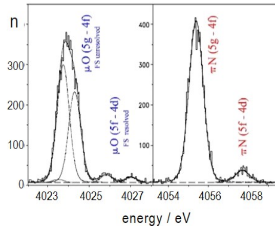
Figure 10.3: \pi N and \mu O(5g-4f) transitions from the simultaneous measurement with an O_2/N_2 (10%/90%) gas mixture at 1.4 bar pressure (adapted from [8]).
