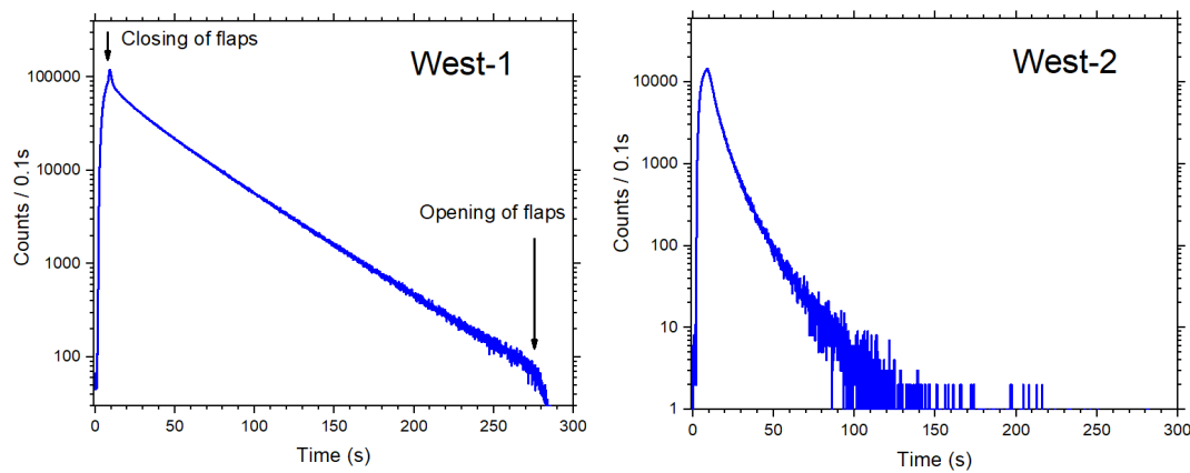
Figure 4.5: a) UCN counts after one proton beam pulse at the West-1 beam port. Closing and opening of the flaps refers to the central flapper valves. b) Same as a) but at the West-2 beam port.
