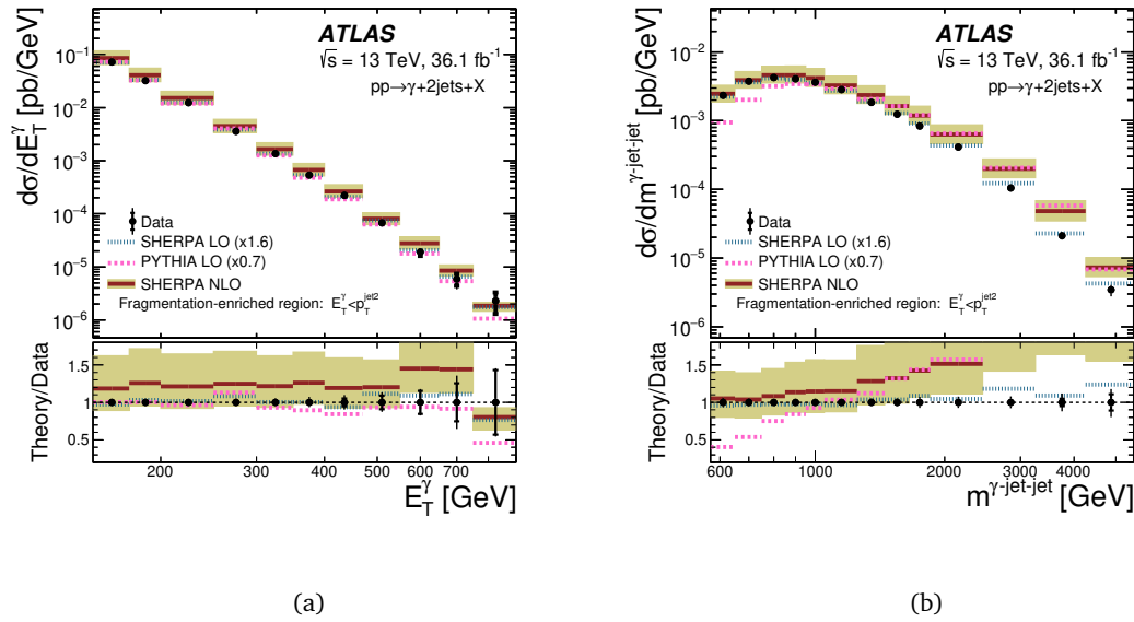
Figure 1: Differential cross-sections of the photon + 2 jet production measured as a function of Figure E_T^\gamma (a) and m_{\gamma\text{-jet-jet}} (b) for both direct and fragmentation process and compared to the theoretical MC predictions [2].
