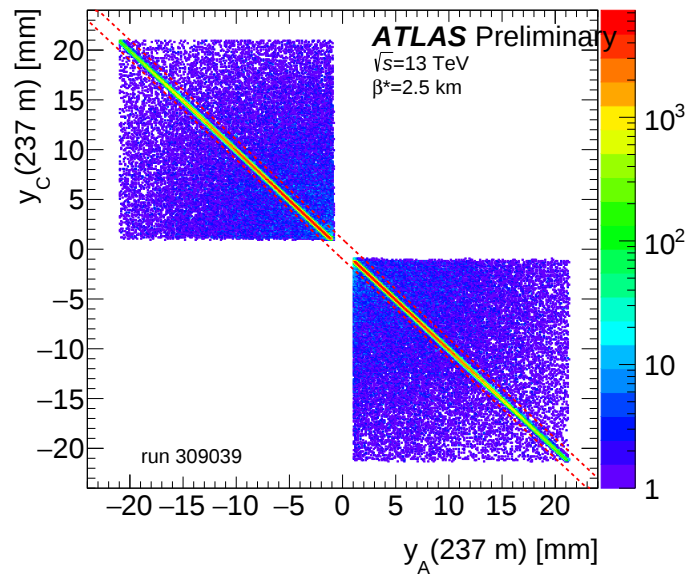
Figure 4: Selecting elastic events from correlation between y -values [1].
