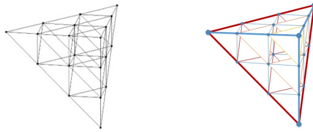
Figure 1: Symmetric \underline{20} ; left: construction by \underline{4} of SU(4) [8], F.6; right: subdivision by Hilbert [16], §19.
