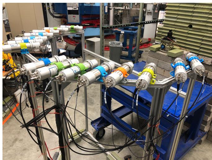
Figure 1: Experimental setup at TUNL
