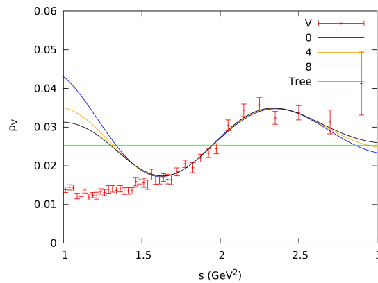
Figure 5: Vector spectral function \rho_V(s) , fitted above 1.55 \text{ GeV}^2 with the ansatz (14), for different values of \lambda_V = 0, 4, 8 , compared with the data points [16]
