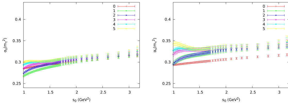
Figure 3: \alpha_s(m_\tau^2) determinations with FOPT (left) and CIPT (right), at different values of s_0 and from different (V + A) A^{(2,m)}(s_0) moments ( 0 \leq m \leq 5 ), ignoring all non-perturbative effects [16]. Only experimental uncertainties are displayed.
