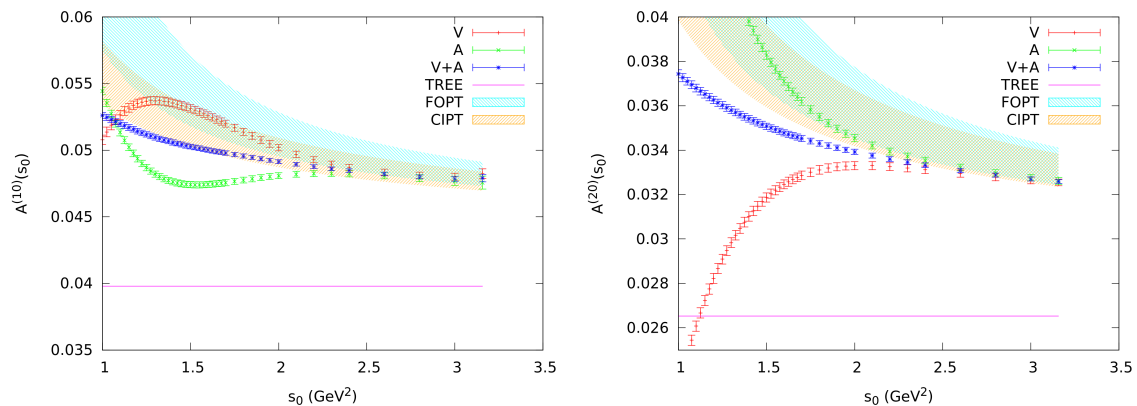
Figure 2: Dependence on s_0 of the experimental moments A^{(1,0)}(s_0) (left) and A^{(2,0)}(s_0) (right), for the V (red), A (green) and \frac{1}{2}(V+A) (blue) channels. The orange and light-blue regions are the CIPT and FOPT perturbative predictions for \alpha_s(m_\tau^2) = 0.329^{+0.020}_{-0.018} [16].
