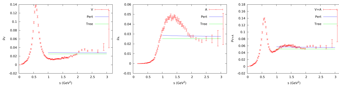
Figure 1: ALEPH spectral functions for the V , A and V + A channels [8].
