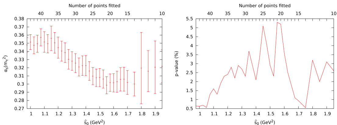
Figure 4: FOPT determination of \alpha_s^{(n_f=3)}(m_\tau^2) from the s_0 dependence of A_V^{(00)}(s_0) , fitting all s_0 bins with s_0 > \hat{s}_0 , as function of \hat{s}_0 , using the approach of Ref. [24].
