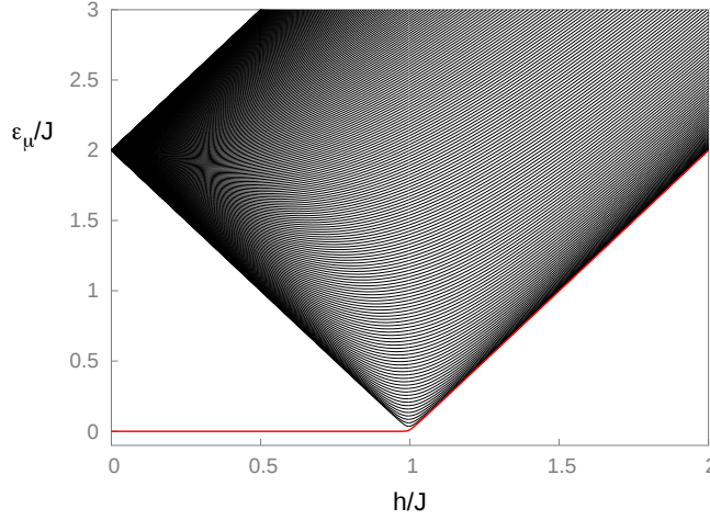
Figure 10: The spectrum of eigenvalues \varepsilon_\mu = 2\varepsilon_\mu \geq 0 of an ordered Ising chain with OBC, versus the transverse field h . (We show only half of the particle-hole symmetric spectrum \pm\varepsilon_\mu .) Here L = 256 . Notice the zero-energy eigenvalue for h < h_c = J . This eigenvalue is exponentially small in the length L for all h < h_c .
