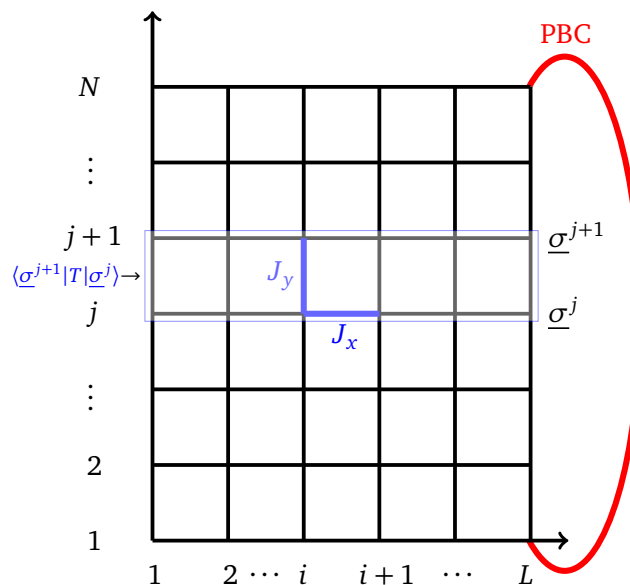
Figure 5: The 2-dimensional classical Ising model on a square lattice with L \times N sites, denoted as (i, j) with 1, \dots, L and j = 1, \dots, N . PBC are enforced in the y -direction: You can think of the system as “living on a cylinder” with axis along the x -direction. Boundary conditions along the x -direction are left unspecified: They could be open , fixed , or periodic . In the latter case, you might picture the system as “living on a torus”. The blue lines highlight the couplings J_x , connecting sites (i, j) and (i + 1, j) , and J_y , connecting (i, j) and (i, j + 1) . The shaded rectangle highlights the Boltzmann weights included in the definition of the “transfer matrix” \langle \underline{\sigma}^{j+1} | T | \underline{\sigma}^j \rangle .
