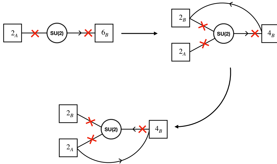
Figure 17: Explanation of SU(6) \times SU(2) \rightarrow E_6 enhancement from Seiberg duality.
