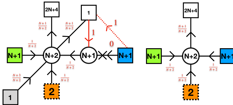
Figure 58: The relations between two trinions. On the left the trinion of Figure 57 glued to the two punctured sphere. The SU(N+1) gauging has N+2 flavors and thus it S-confines to give a WZ model of mesons and baryons. The mesons charged under SU(N+1) puncture symmetry becomes a bifundamental under puncture and SU(N+2) gauge symmetry. The meson built from the \Phi -field (denoted by red line) gives mass to one of the 2N+5 fundamentals. The baryon gives mass to the field charged under U(1) symmetry (denoted by shaded grey on the quiver). Finally, we have a baryon built from the bifundamental and the \Phi field denoted by red solid line which gets a mass with the dashed red line. This theory then flows to the one on the right side. The Figure is taken from [25].
