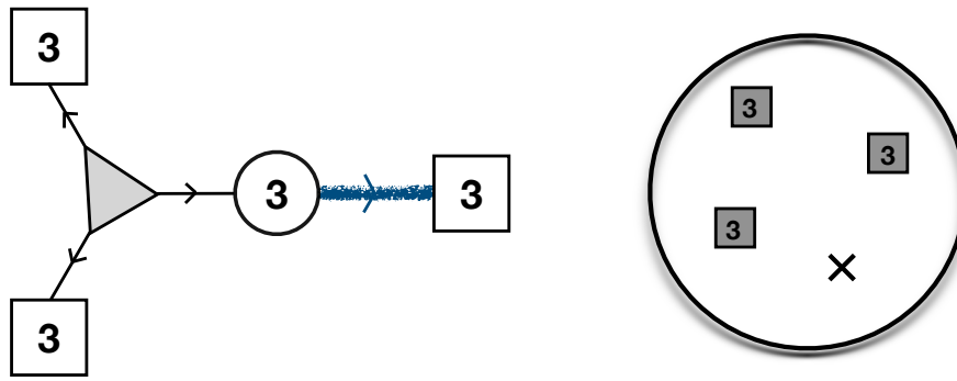
Figure 28: Closing a puncture of the four punctured sphere. The squares are SU(3) punctures and crosses are empty ones. On the conformal manifold at most two SU(3) symmetries are preserved. On a general locus all symmetry is broken and the model can be interpreted as a model with ten empty punctures.
