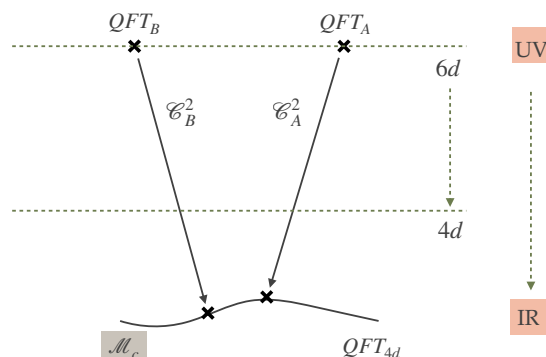
Figure 4: A depiction of a 6d duality. Starting from two different theories in 6d and deforming them by different geometries one can flow to equivalent theories in 4d.
