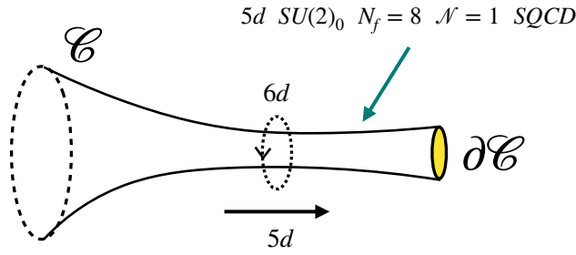
Figure 30: Compactifying the 6d rank one E-string on a circle with a certain holonomy breaking the E_8 symmetry to SO(16) is conjectured to be described in 5d by an effective theory which is SU(2) SQCD with eight flavors. The UV completion of the 5d theory is the 6d SCFT. Here \mathcal{C} is the Riemann surface and \partial\mathcal{C} is non empty, we have a puncture.
