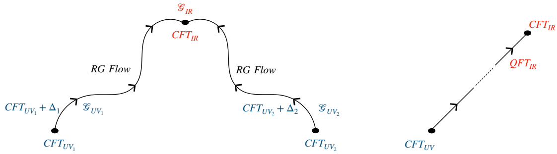
Figure 12: A depiction of IR dualities. On the left we have two different UV CFTs deformed to flow to the same IR fixed point. On the right we have a UV CFT deformed (e.g. a weakly coupled asymptotically free gauge theory) flowing in the IR to a QFT which close to the IR fixed point can be described by yet another weakly coupled theory (e.g. an IR free gauge theory).
