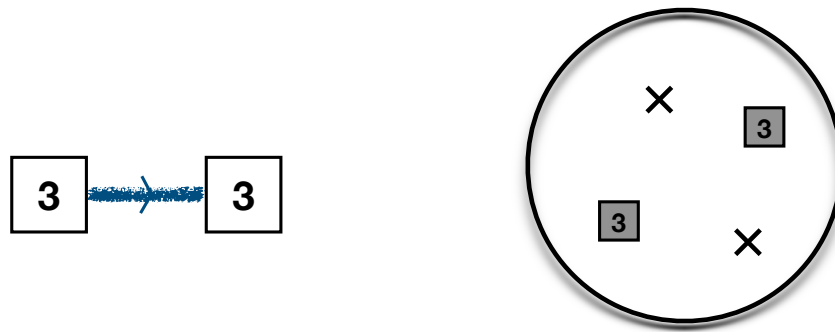
Figure 29: Closing SU(3) puncture of Fig. 5 we obtain a Wess-Zumino theory with two SU(3) and two empty punctures.
