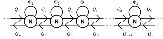
Figure 9: The necklace quiver of length n .
