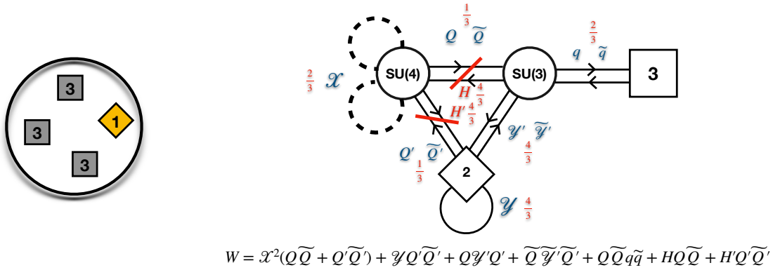
Figure 64: The theory corresponding to a sphere with three maximal punctures and one minimal puncture obtained by gluing to a T_3 the free trininion. On the right we have a non-conformal description of the theory using the Lagrangian of [82] for the T_3 . The fields H and H' are gauge singlets, and Y is adjoint of SU(2) . One maximal puncture SU(3) and the minimal puncture U(1) are manifest in the UV, while the remaining two maximal puncture SU(3) symmetries emerge in the IR enhancing an SU(2)^2 \times U(1)^2 symmetry of the Lagrangian. The U(1)_t symmetry is conjectured to emerge in the IR. One can further turn on marginal deformations consistent with the R-symmetry assignment in the Figure breaking completely all the global symmetry.
