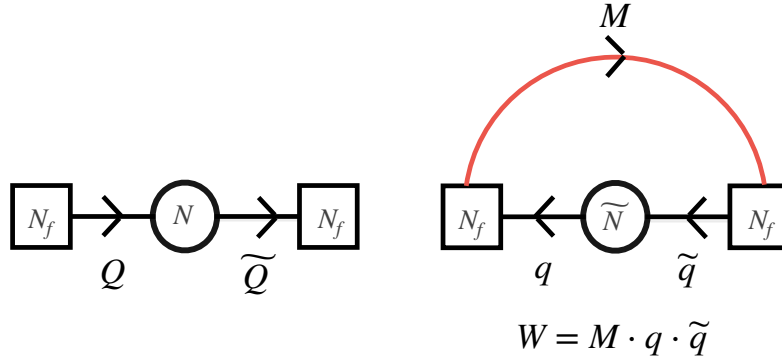
Figure 13: A depiction of Seiberg duality with SU(N) gauge groups.
