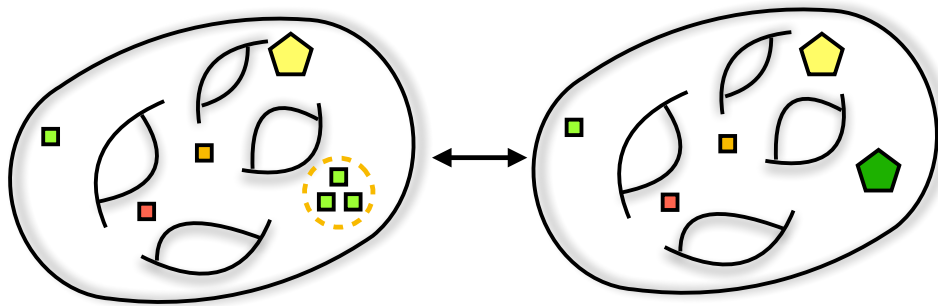
Figure 60: Atypical degenerations of the surface. In numerous examples in certain limits of collision of some types of punctures one can obtain a new type of a puncture. The symmetry of the new “composite” puncture might be different than the symmetry of the punctures building it. Conversely, there are examples of exactly marginal deformations breaking the puncture symmetry and not corresponding to naive geometric deformations of the surface.
