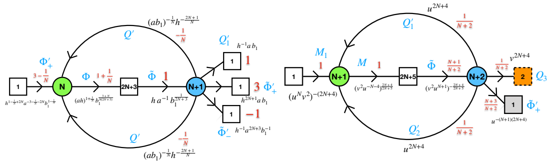
Figure 55: On the left the quiver obtained after the flow using the UV fugacities (dropping the gauge singlet fields). On the right the quiver with redefined (and simplified) definitions of symmetries. We have also shifted N by one on the right side to switch again to the notations with N = 1 corresponding to the E-string.
