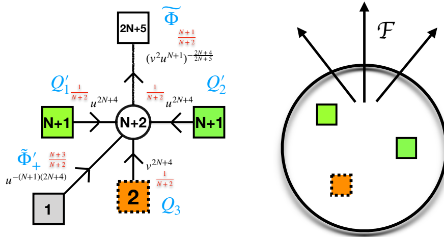
Figure 57: The three punctured sphere obtained by cutting the cycle of the one punctured torus. We have a baryonic superpotential \tilde{\Phi}'_+ \cdot (Q_1'^{N+1} + Q_2'^{N+1}) , which is irrelevant but the case of N = 1 . The trinion is associated to flux (-2, 0, \dots) which preserves U(1) \times SO(4N + 10) symmetry. The Figure is taken partially from [25].
