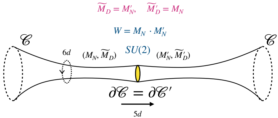
Figure 36: Explanation of S-gluing in 5d. We have the 16 fields on the left (M_N, \tilde{M}_D) and on the right, (M'_N, \tilde{M}'_D) . We gave eight of these Dirichlet (label D ) and eight Neumann (label N ) boundary conditions. Now we are undoing the boundary conditions by gauging the SU(2) symmetry and identifying M'_D with M_N and M_D with M'_N , and thus having the full set of dynamical fields at the four dimensional boundary given by M_N and M'_N .
