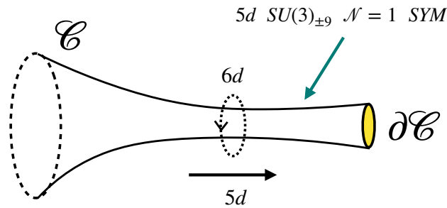
Figure 23: Compactifying the 6d SU(3) minimal SCFT on a circle with the complex conjugation twist is conjectured to be described in 5d by an effective theory which is SU(3) SYM with level \pm 9 CS term. The UV completion of the 5d theory is the 6d SCFT. Here \mathcal{C} is the Riemann surface and \partial\mathcal{C} is non empty, that is we have a puncture. Each puncture is associated with a global symmetry corresponding to the 5d gauge symmetry, which is SU(3) in this case.
