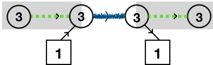
Figure 27: An equivalent way to depict the dumbbell quiver. The two shaded sub-quivers are \mathcal{N} = 4 SYM. As \mathbf{3} \times \bar{\mathbf{3}} = \mathbf{8} \oplus \mathbf{1} two trifundamental fields split to (\mathbf{8}, \mathbf{3}) and (\mathbf{1}, \mathbf{3}) of SU(3) \times SU(3) . The dotted lines represent a triplet of adjoints of SU(3) .
