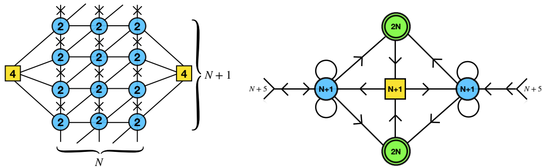
Figure 61: On the left we have the theory obtained by compactifying (D_{N+3}, D_{N+3}) minimal conformal matter theory on a torus with one unit of flux breaking the SO(4N + 12) symmetry of the 6d SCFT to U(1) \times SU(N + 1) \times SO(10 + 2N) . On the right we have a dual theory [19] (double circles correspond to USp groups and the lines starting and ending on the same vertex are in antisymmetric representation). We assume that N is an odd integer. Note the two dual theories manifest different subgroups of the global symmetry group. The model on the right is obtained by gluing two tubes with USp(2N) and SU(N + 1) punctures while on the left we glue tubes with SU(2)^N punctures. This duality follows from a 5d UV duality. The theory on the left (removing the free flip fields) can be alternatively obtained by compactifying the SCFT on two M5 branes probing \mathbb{Z}_{N+1} singularity on a sphere with two maximal and N + 1 minimal punctures: This is thus an example of a 6d duality.
