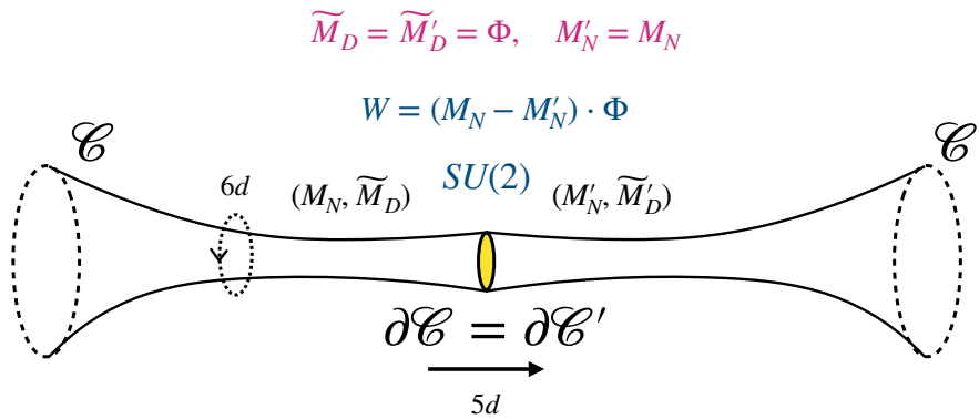
Figure 39: Explanation of \Phi -gluing in 5d. We have the 16 fields on the left (M_N, \tilde{M}_D) and on the right, (M'_N, \tilde{M}'_D) . We gave eight of these Dirichlet (label D ) and eight Neumann (label N ) boundary conditions. Now we are undoing the boundary conditions by gauging the SU(2) symmetry and identifying M'_D with M_D and \Phi and M_N with M'_N , and thus having the full set of dynamical fields at the four dimensional boundary given by \Phi and M_N = M'_N .
