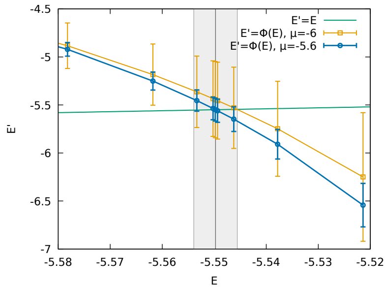
Figure 16: Energy estimation using the self-energy in imaginary time with \phi(E) , the right hand side of Eq. 17. Same parameters are used as before ( \alpha = 5 ; \mu = -6 and \mu = -5.6 , respectively). The intersection point with the E' = E line determines the polaron ground state energy. It is marked for the case of \mu = -5.6 and its error bars are given by the gray area.
