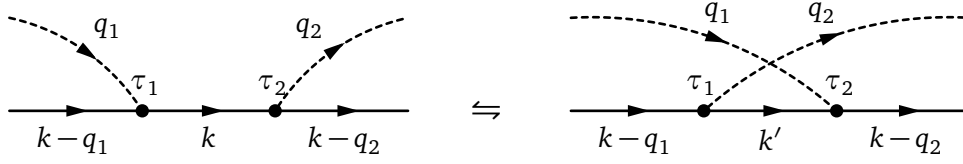
Figure 7: Illustration of the SWAP update. The phonon propagators carrying momentum q_1 and q_2 are understood to connect back to the fermion line at vertices at times \tau_A and \tau_B , respectively. \tau_A and \tau_B may each be either before or after \tau_1 and \tau_2 . After the update, the central fermion propagator carries a momentum k' = k - q_1 - q_2 .
