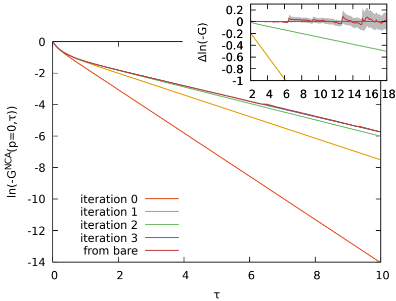
Figure 18: The Green function G^{\text{NCA}}(p=0, \tau) in the non-crossing approximation for \alpha = 5 and \mu = -4 . Shown are the first 4 iterations with the initial guess G = G_0 and compared with the result obtained by sampling the corresponding diagrams in the bare expansion. We used 256 points in imaginary time on a logarithmic grid and 2^{13} Matsubara frequencies. We took 200 equidistant points in momentum space with a momentum cutoff at k_c = 100 . The results are obtained in just a few minutes on a single core. The inset shows the residues after subtracting the result after 4 iterations. The error bars on the Green function sampled from the bare expansion are indicated by the area shaded in gray.
