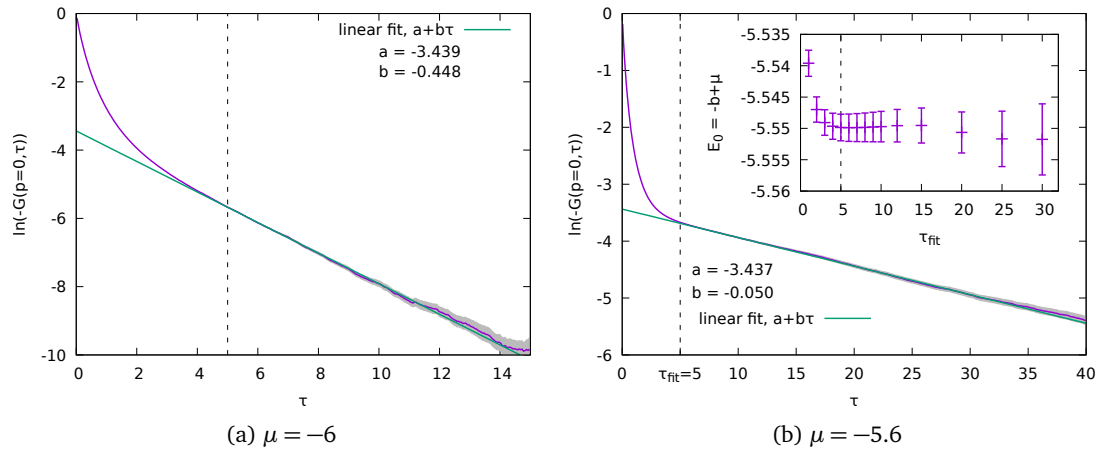
Figure 9: Logarithm of the Green function \ln(-G(p=0, \tau)) as a function of imaginary time \tau for \alpha = 5 and different values of \mu . Error bars are indicated by the shaded area. The exponential decay of the Green function is fitted starting from \tau_{\text{fit}} = 5 in order to obtain the polaron ground state energy and its residue, cf. Eq. 21. The inset in panel (b) shows the polaron energy (computed from the slope of the fit) for different fit windows [\tau_{\text{fit}}, 40] . Error bars on these data have been obtained by considering 28 independent simulations. One can see that \tau_{\text{fit}} = 5 is sufficiently great to probe the asymptotic regime. We switched off the CHANGE-P update and used a uniform grid in the \tau -direction. The code ran for 36 (a) and 467 (b) CPU-hours with the number of updates totalling 10^{12} and 10^{13} respectively.
