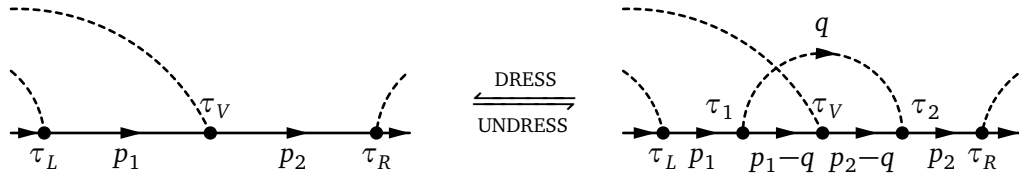
Figure 23: Illustration of the VERTEX-DRESS / VERTEX-UNDRESS pair of updates.
