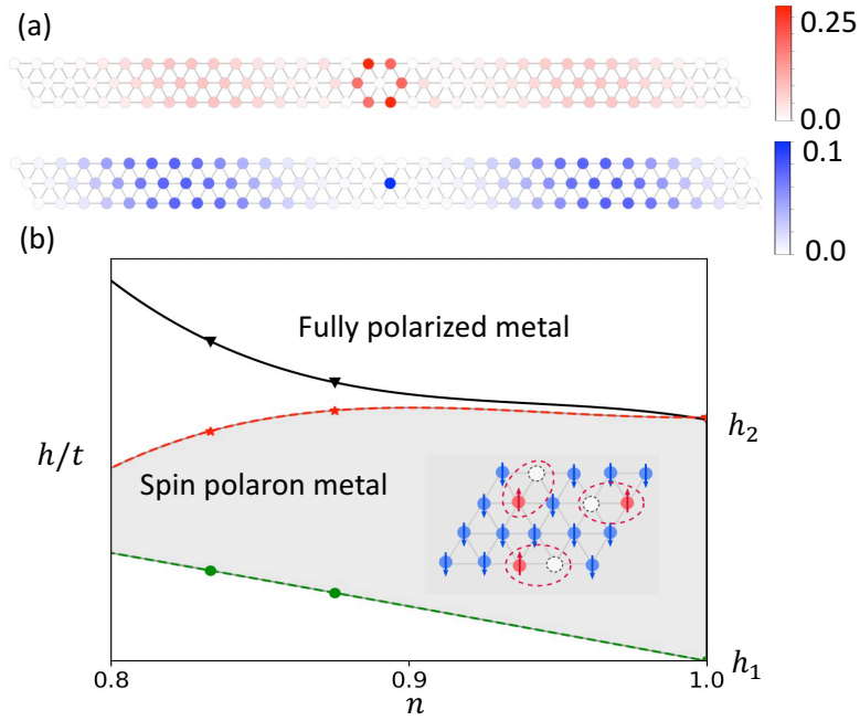
Figure 2: (a) Hole-spin correlation function C_{hs}(i, o)/\delta in a 33 \times 3 cylinder with 3 spin polarons, where holes are tightly bounded to the spin flips. The bottom panel is the Hole-Hole correlation function C_{hh}(i, o)/\delta . o is the center of cylinder. (b) Schematic figure of doping- and field-dependent phase diagram. The data points are taken from DMRG on a 24 \times 3 cylinder. Here N is the number of sites and Nh is the number of holes.
