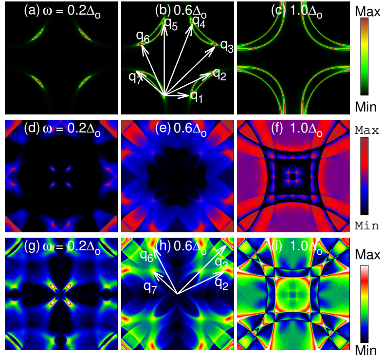
Figure 1: (a-c) The CECs for the quasiparticle energies in steps of 0.4\Delta_o within the range 0 \leq \omega \leq \Delta_o . The banana-shaped CECs can be seen to exist up to \Delta_o . (d-f) g -maps and (g-i) z -maps for various quasiparticle energies in similar steps when a non-magnetic impurity is present. The QPI patterns are dominated by the scattering vectors \mathbf{q}_2 , \mathbf{q}_3 , \mathbf{q}_6 , and \mathbf{q}_7 . There is no significant difference between the two sets of map.
