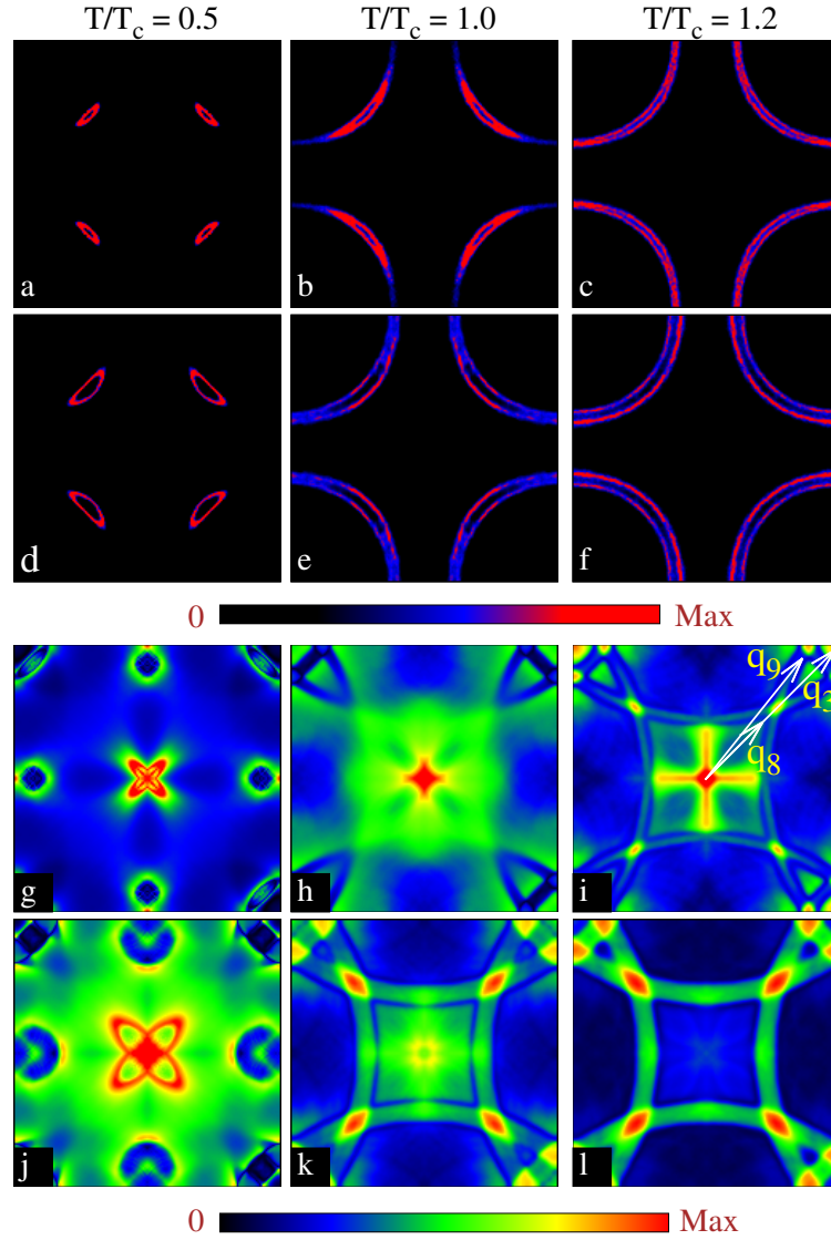
Figure 3: Evolution of quasiparticle spectral function \mathcal{A}(\mathbf{k}, \omega) for \omega = (a-c) 0.15t and (d-f) 0.3t as a function of temperature. k_x and k_y are along horizontal and vertical directions, respectively, with each having range [-\pi, \pi] . Corresponding QPIs for \omega = (g-i) 0.15t and (j-l) 0.3t .
