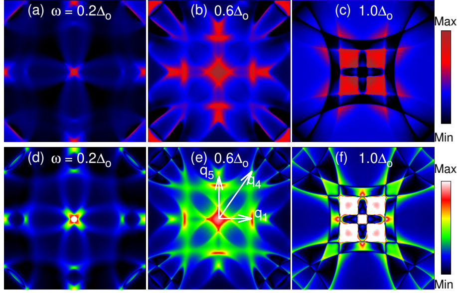
Figure 2: (a-c) g -maps and (d-f) z -maps for the quasiparticle energies in steps of 0.4\Delta_0 when the impurity atom is magnetic. The patterns have enhanced features corresponding to the scattering vectors \mathbf{q}_1 , \mathbf{q}_4 , and \mathbf{q}_5 .
