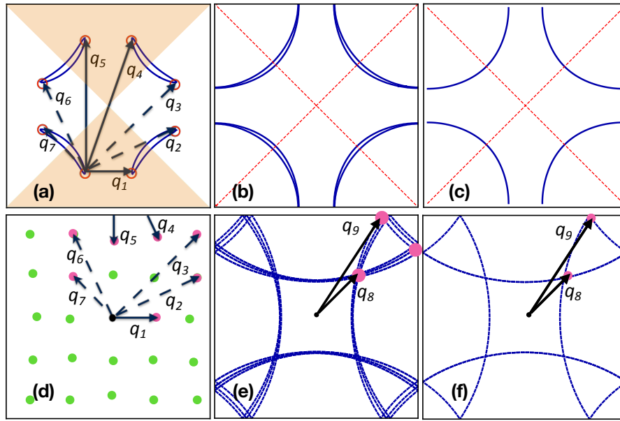
Figure 4: (a) The schematics of the banana-shaped CECs in the d -wave superconducting state. The CECs at non-zero (b) finite energy \omega \gtrsim \Delta_{an} in the temperature regime T_c < T < T^* or when T > T^* and (c) \omega = 0 . The scattering vectors \mathbf{q}_8 and \mathbf{q}_9 are mainly responsible for the QPI patterns at high energy and high temperature. (d), (e) and (f) indicate scattering vectors and corresponding patterns.
