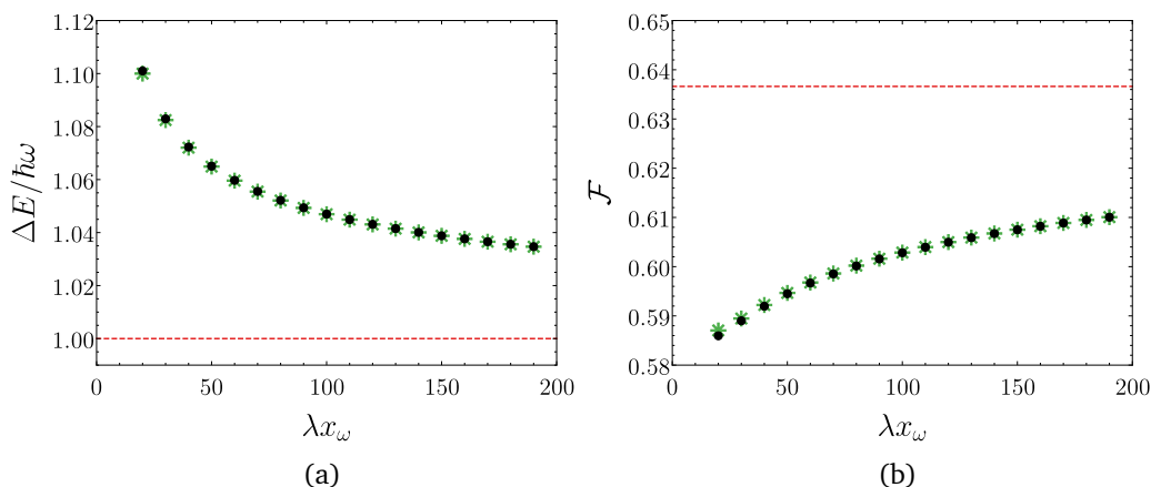
Figure 1: a) Energy for two pairs, excluding the trivial contribution equal to twice the single-pair energy, as a function of \lambda . b) Fidelity between the coboson ansatz and the numerically found ground state as a function of \lambda . The results are obtained from the lowest non-trivial order of the Taylor expansion (green stars) and the next non-zero higher-order corrections (black circles) as reported in Appendix A. The horizontal dashed red lines indicate the asymptotic values for \lambda \rightarrow \infty .
