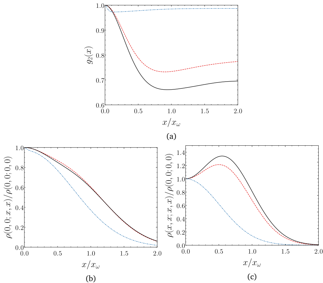
Figure 5: a) Off-diagonal correlation function g_2(x) , b) off-diagonal matrix elements and c) diagonal matrix elements of the reduced density matrix \rho_{ab} . Black solid lines correspond to numerical results for \lambda x_\omega = 30 , red dashed ones to point-like hard-core bosons and blue dash-dotted lines correspond to the prediction of the coboson ansatz for N = 2 and \lambda x_\omega = 30 . Details are provided in the main text and in Appendix D. Notice that the vertical axis of subplot (a) does not begin at zero.
