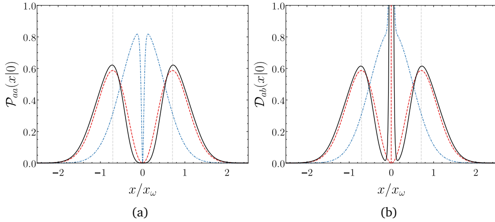
Figure 4: a) Conditional probability \mathcal{P}_{aa}(x|0) to find a fermion of kind a at position x when another fermion was already found at the origin. b) Conditional density \mathcal{D}_{ab}(x|0) indicating the density of fermions of kind a at position x conditioned on having found a fermion of kind b at the origin. In both plots the solid black curve is the numerical result with \lambda x_\omega = 30 and n_{\max} = \lambda x_\omega . The dashed red curve is the analytical result for the probability obtained for the point-like hard-core boson limit, and the blue dash-dotted line is the probability predicted by the coboson ansatz in Eq. (12) for N = 2 and \lambda x_\omega = 30 . Details of the calculations are given in Appendices B and C. The vertical light-gray lines indicate the positions \pm x_\omega/\sqrt{2} , which are the locations of the maxima of the conditional probability for \lambda \rightarrow \infty .
