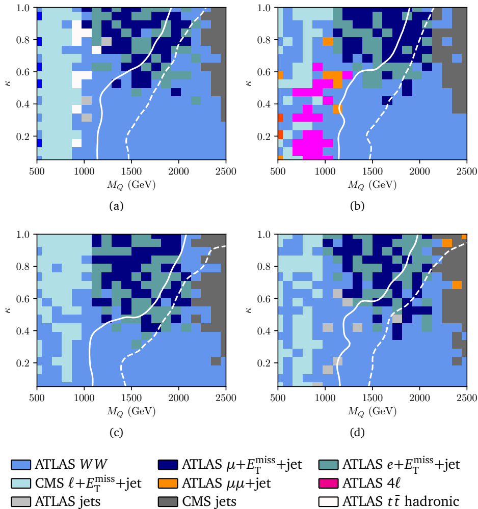
Figure 23: Dominant LHC analysis pools contributing to VLQ limit-setting in the \kappa vs VLQ mass plane, where \kappa is the coupling to third-generation SM quarks, without bin-to-bin correlations included in the \text{CL}_s calculations. All VLQ ( B, T, X, Y ) masses are set to be degenerate. The disfavoured regions are located above and to the left of the dashed (68% CL) and solid (95% CL) white contours respectively. The VLQ branching fractions to W:Z:H are (a) 0:0:1 (b) 0:1:0 (c) 1:0:0 and (d) \frac{1}{2}:\frac{1}{4}:\frac{1}{4} .
