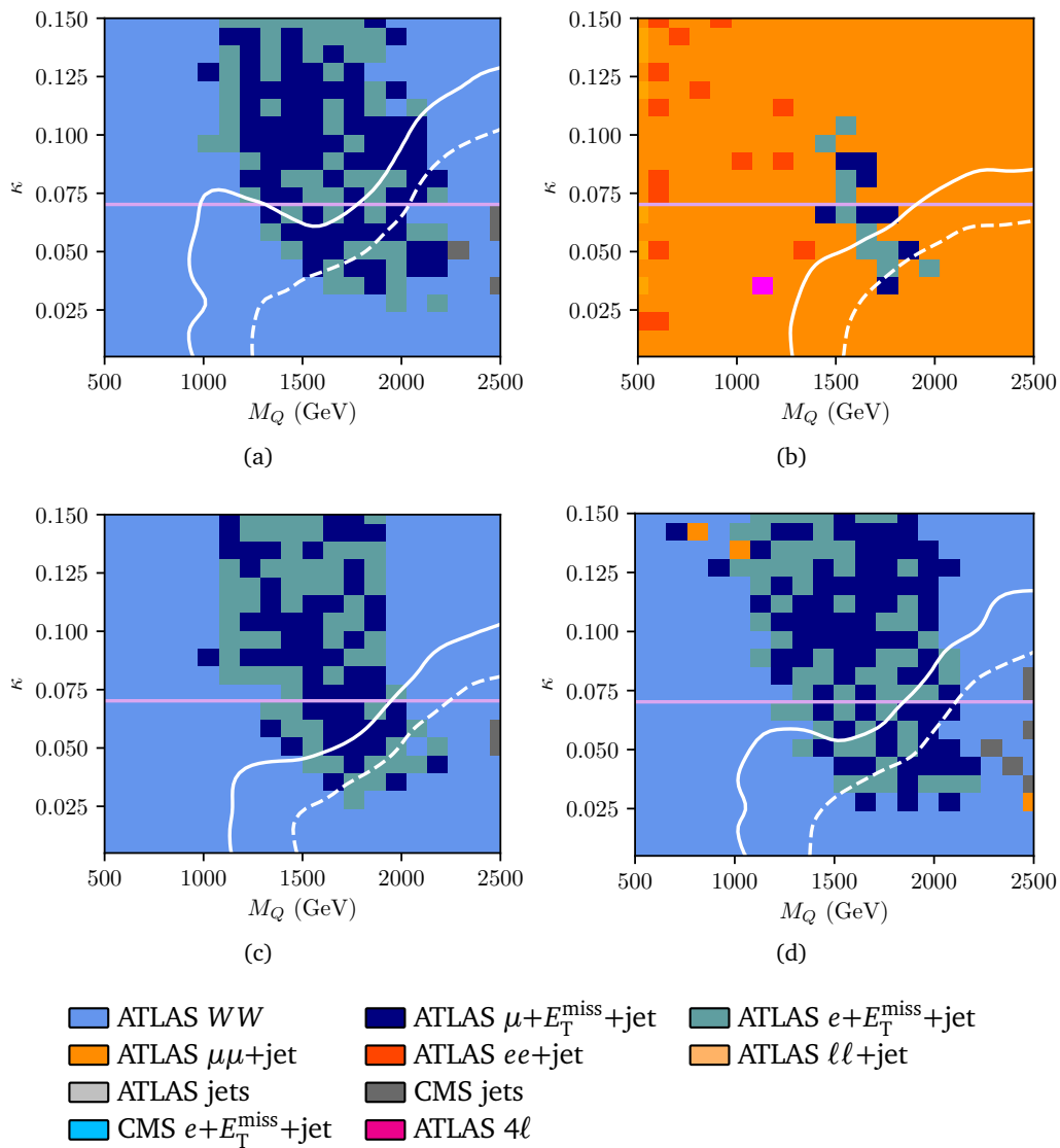
Figure 7: Dominant LHC analysis pools contributing to VLQ limit-setting in the \kappa vs VLQ mass plane, where \kappa is the coupling to first-generation SM quarks. All VLQ ( B, T, X, Y ) masses are set to be degenerate. The disfavoured regions are located above and to the left of the dashed (68% CL) and solid (95% CL) white contours respectively. The lower bounds in \kappa from non-LHC flavour physics are indicated with the pink horizontal contour. The VLQ branching fractions to W:Z:H are (a) 0:0:1 (b) 0:1:0 (c) 1:0:0 and (d) \frac{1}{2}:\frac{1}{4}:\frac{1}{4} .
