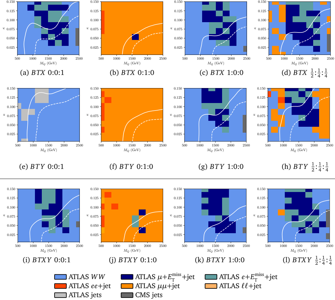
Figure 11: Sensitivity of LHC measurements to VLQ triplet production in the \kappa vs VLQ mass plane, where \kappa is the coupling to first-generation SM quarks. All VLQ masses are set to be degenerate. The multiplets are given as rows: (a)–(d) (B, T, X) triplet, (e)–(h) (B, T, Y) triplet, and for comparison to the main text, the (i)–(l) (B, T, X, Y) quadruplet. The VLQ branching fractions to W:Z:H are arranged in columns of 0:0:1, 0:1:0, 1:0:0, and \frac{1}{2}:\frac{1}{4}:\frac{1}{4} from left to right.
