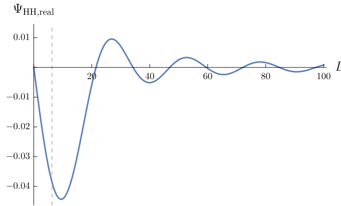
Figure 4: Plot of the wavefunction \Psi_{\text{HH,real}} for \phi_b = 1/4 . The vertical dashed line indicates the location, L = 2\pi , where the expanding branch \Psi_+ of the wavefunction (102) diverges, but \Psi_{\text{HH,real}} remains finite.
