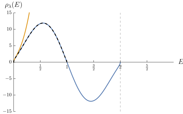
Figure 2: In orange, we show the undeformed density of states \sinh(2\pi\sqrt{E}) of JT gravity at infinite cutoff. In dashed black, we show the density of states of the theory with just the branch of the root, \mathcal{E}_- , that connects to the undeformed energies, until the energy complexifies. In blue, we show the density of states \rho_\lambda(E) of the deformed partition function (89) which includes non-perturbative corrections in \lambda . Above we have set \hat{\rho}(E) = 0 and \lambda = 1/4 and C = 1/2 , the black line therefore ends at E = \frac{1}{4\lambda} = 1 . The vertical dashed line indicates the energy beyond which \hat{\rho} has support.
