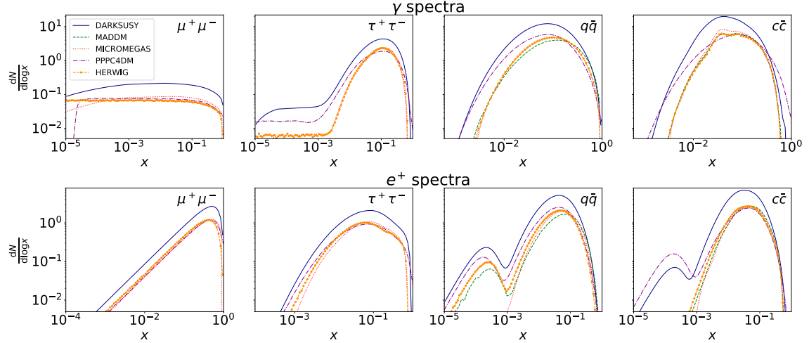
Figure 1: Photon and positron spectra dN/d \log x with x = E_{\text{kin}}/m_\chi for m_\chi = 5 GeV from the different hard annihilation channels. We show results from DARKSUSY, MADDM, MICROMEGAS, PPC4DMID, and HERWIG.
