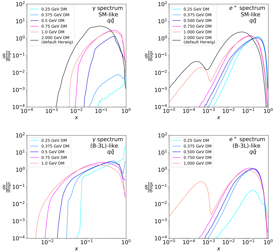
Figure 3: Photon and positron spectra dN/d\log x with x = E_{\text{kin}}/m_\chi for m_\chi = 0.25 \dots 2 GeV from u, d, s, c quarks with SM-like and (B-3L) -like couplings. We use our modified version of HERWIG7 for all curves below 2 GeV.
