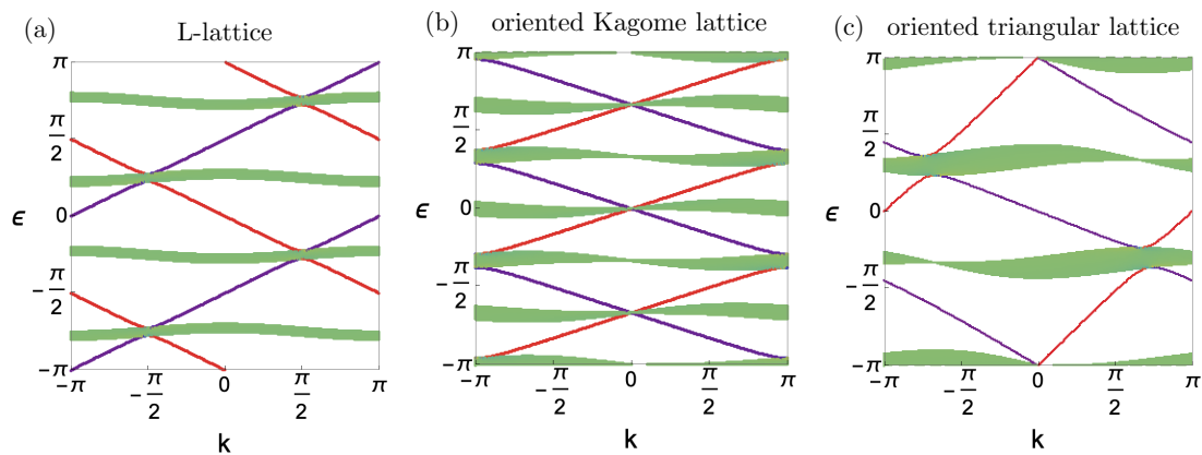
Figure 4: Eigenvalue phase spectrum \epsilon of the "one-step" Chalker-Coddington evolution operator (9) for three cyclic oriented lattices in a cylinder geometry, slightly away from strong phase rotation symmetric point, as a function of the quasi-momentum in the direction parallel to the edges of the cylinder. The color code represent the mean position in the corresponding eigenstate, from one edge (red) to the other (blue) through the bulk (green).
