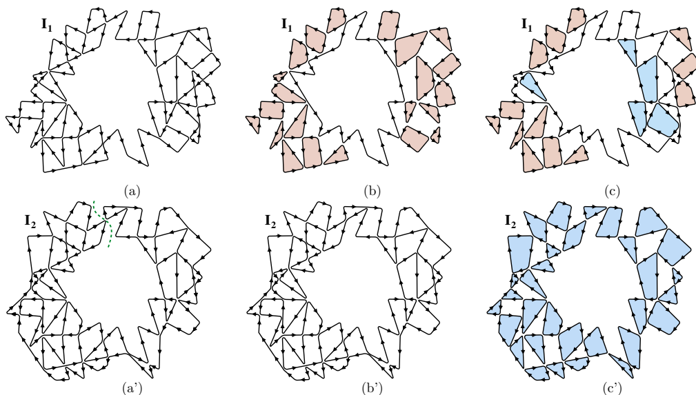
Figure 9: Interface graph I_1 (top) and I_2 (bottom). (a) and (a') are Eulerian circuits that wind and does not wind respectively around the central face. (b') decomposition of I_2 into a clockwise and a counter clockwise circuits. (b) and (c) are examples of non-minimal Veblen decompositions of I_1 . (c') is the minimal Veblen decomposition of I_2 .
