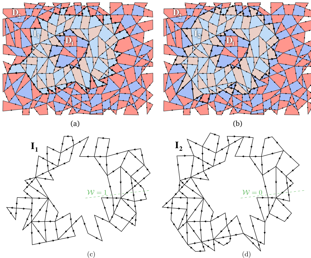
Figure 8: Eulerian graph \mathcal{E} . Each face is assigned to a color or equivalently to an orientation (red + and blue -). (a) Circuits C_1 and C_2 have the same circulation (clockwise). (b) Circuits C_1 and C_2 have opposite circulation. The domain D_1 is the same in (a) and (b). (c) and (d): the two interface graphs \mathbf{I}_1 and \mathbf{I}_2 extracted from figures (a) and (b) respectively (and slightly enlarged for clarity) have different winding numbers.
