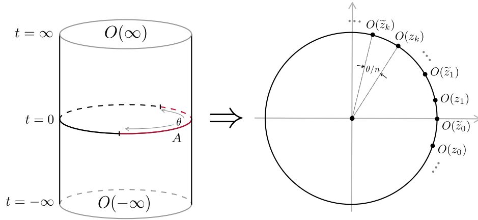
Figure 2: Geometry of our set-up. Left : The geometry before the uniformization map. The operators O are inserted at \pm\infty to create |\psi\rangle and \langle\psi| . The region A of length \theta is displayed in red. Right : Clockwise arrangement of operators along the unit circle in the replicated theory after uniformization and a conformal map to the plane. The distance between the operators at z_k and \tilde{z}_k along the unit circle is \theta/n , the interval length divided by n .
