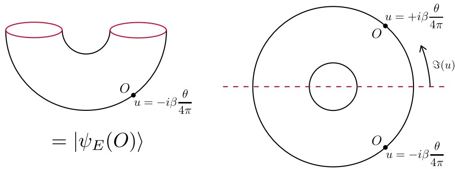
Figure 5: Path integral representation of the state |\psi_E(O)\rangle and its norm in u coordinates. Left : Path integral representation of the state |\psi_E(O)\rangle in the extended Hilbert space. Right : The norm of |\psi_E(O)\rangle . The red dashed line indicates where we cut the u -torus open.
