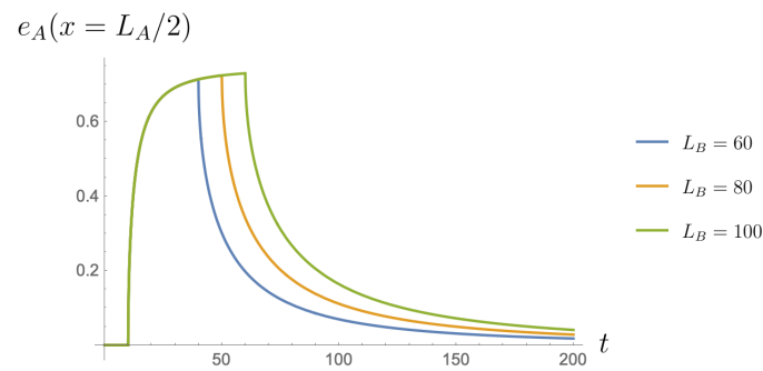
Figure 8: The negativity contour for the free fermion Hamiltonian (C74). We take L_A = 40 to provide the same parameters as Fig. 5 which has a very similar form. The late-time decay is proportional to t^{-2} . Note that the time scales for this model are twice that of the SSH quench due to the factor of two difference in the low energy dispersion relations of the models.
