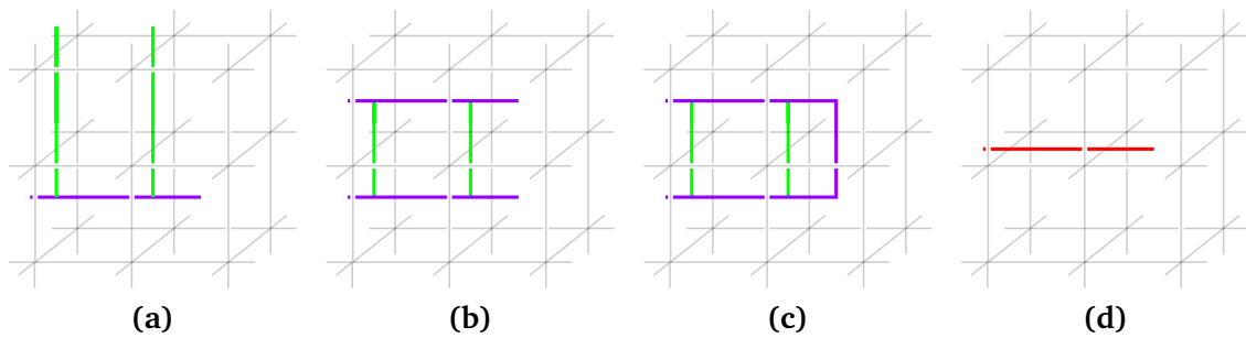
Figure 8: (a) An open string (dual to the membranes), which corresponds to a fracton excitation. (b) A fracton diople given by two fractons separated by a plane. It is mobile in the plane orthogonal to the green strings and is therefore a planon. (c) A fracton dipole that differs from (b) by only local excitations. (d) A planon given by an open string in a 2D plane. This is an equivalent excitation to (c) since both break the constraint that a plaquette can be penetrated by a purple string if and only if a red, green, or blue string ends at the plaquette.
