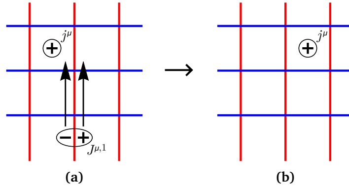
Figure 3: A 2D slice of 3D space showing two foliations (red and blue). (a) When in isolation, a charge (sourced by j^\mu ) cannot move through a foliation layer, which results in the mobility constraints tabulated in Tab. 1. However, a dipole J^{\mu,1} can move along a red layer and be absorbed by the charge to move the charge to the right, as depicted in (b) .
