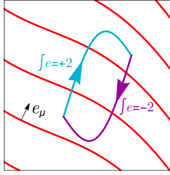
Figure 2: A 2D slice of 3D space showing a single foliation of 2D layers, which appear as red lines in this cross-section. The foliation field e_\mu points orthogonal to the layers such that \int_p e^k \equiv \int_p e_\mu^k dx^\mu counts the number of layers that the path p crosses. In the figure, we show two paths and the resulting integrals. A contractible closed path, e.g. the composition of the cyan and purple paths, results in \oint_p e^k = 0 . In the field theory, the (red) foliating layers are infinitesimally close to each other. A cutoff can be added to allow for a notion of finite layer spacing.
