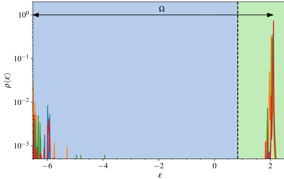
Figure 5: Spectral decomposition of the Floquet multifractal states. The spectral density of states \rho(\epsilon) for typical Floquet multifractal states chosen at random (different colors) show overwhelming contributions from the static eigenstates separated by \epsilon = \Omega . The blue and green shaded regions correspond to the localized and delocalized part of the undriven spectrum, respectively. The black dashed line denotes the mobility edge, states near which do not get affected by the Floquet drive. The parameters correspond to Fig. 2.
