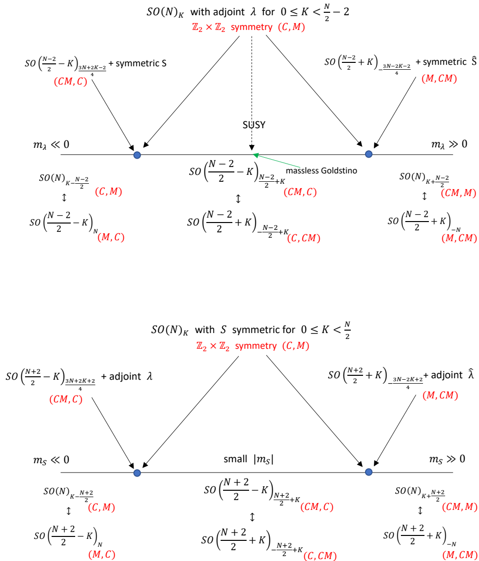
Figure 4: The phase diagrams of SO(N) gauge theory coupled tensor fermions. The infrared TQFTs, together with relevant level-rank duals are shown along the bottom. The blue dots indicate the transitions from the semiclassical phase to the quantum phase. This proceeds through a tensor transition described by a dual theory, which covers part of the phase diagram. At a special value of the mass in the quantum phase of the adjoint theory, a massless goldstino appears. These figures are identical to those in [6] except that we now add the map of the \mathbb{Z}_2 \times \mathbb{Z}_2 global symmetry.
