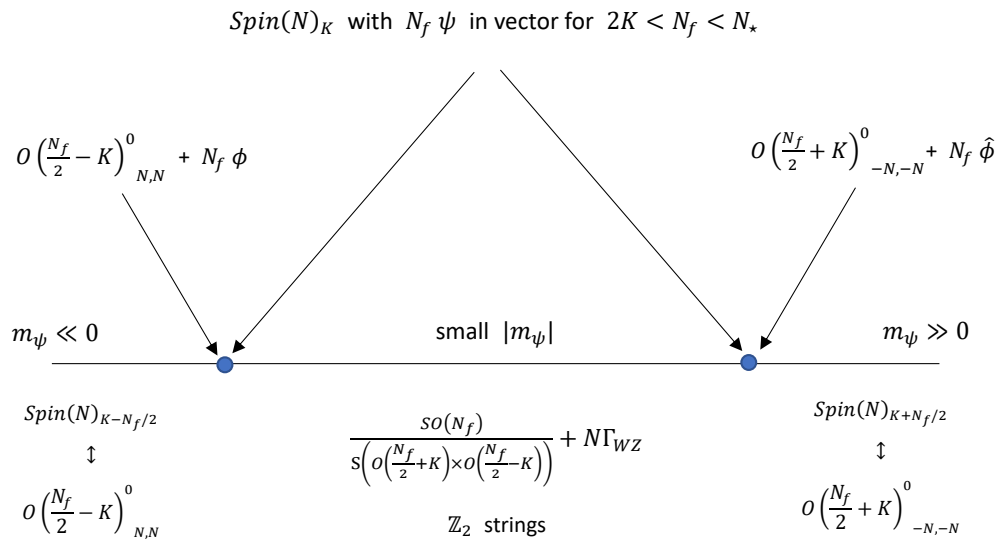
Figure 1: The phase diagram of Spin(N) gauge theory coupled to fermions in the vector representation. For large |m_\psi| the infrared is a topological field theory, which is visible semiclassically. For small |m_\psi| the theory spontaneously breaks the flavor symmetry and is described by a sigma model with Grassmannian target. There is a Wess-Zumino term, and stable strings, signaling confinement. The transition from the semiclassical phase to the quantum phase is weakly coupled in the dual bosonic variables ( \phi or \hat{\phi} ). This diagram completes the discussion in [5] by specifying the discrete \theta -parameters needed in the various gauge theories, and provides a non-trivial consistency check on that proposal.
