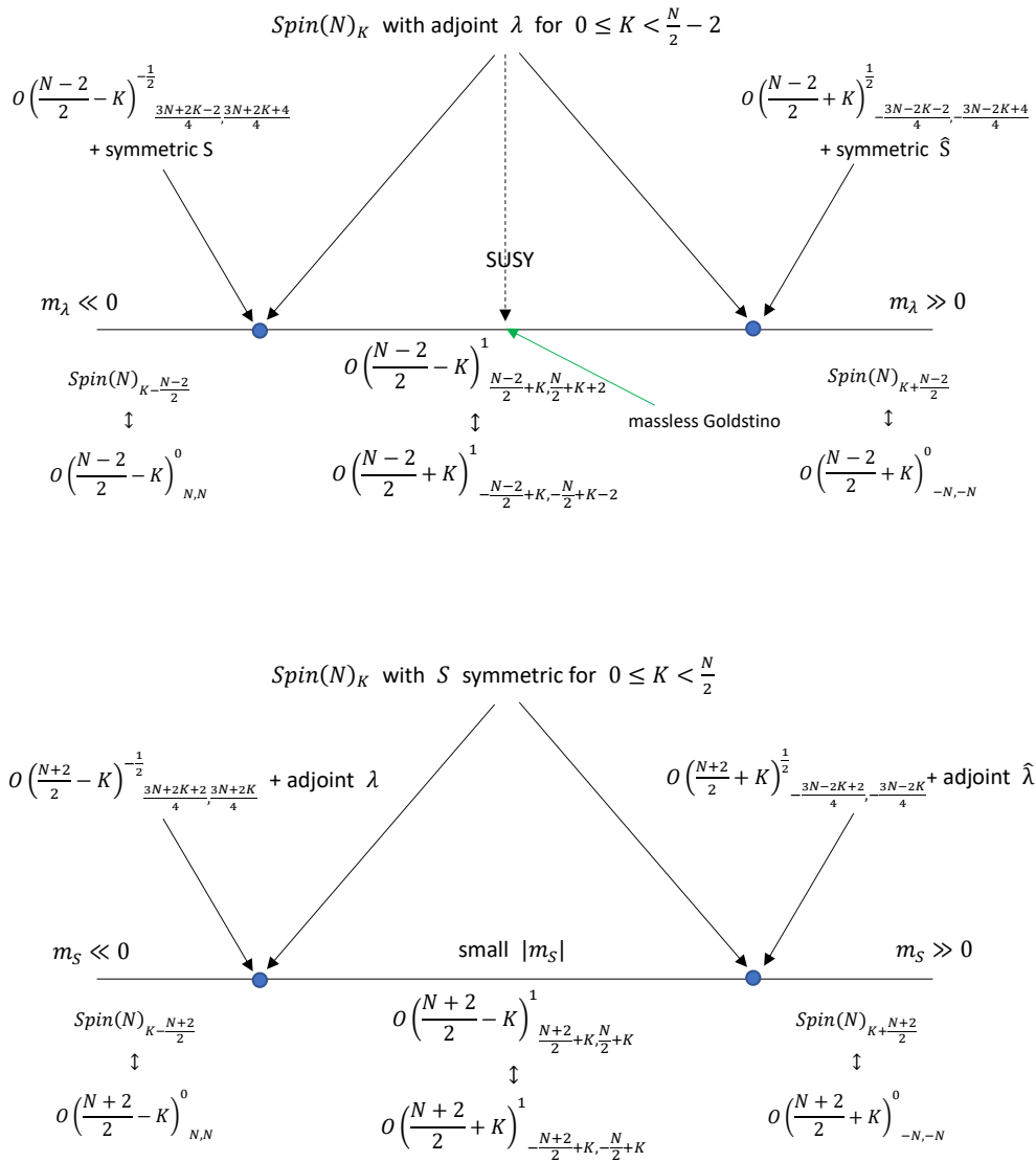
Figure 5: The phase diagrams of Spin(N) gauge theory coupled tensor fermions. The infrared TQFTs, together with relevant level-rank duals are shown along the bottom. The blue dots indicate the transitions from the semiclassical phase to the quantum phase. This proceeds through a tensor transition described by a dual theory, which covers part of the phase diagram. Across these tensor transitions O(L)^0 and O(L)^1 are exchanged. At a special value of the mass in the quantum phase of the adjoint theory, a massless goldstino appears.
