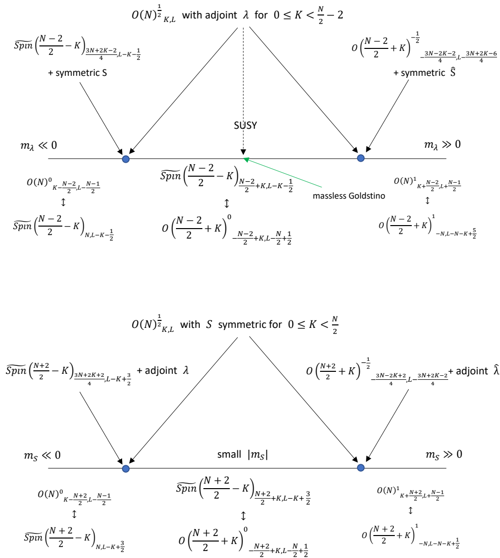
Figure 6: The phase diagrams of O(N)^{\frac{1}{2}} gauge theory coupled tensor fermions. The infrared TQFTs, together with relevant level-rank duals are shown along the bottom. The blue dots indicate the transitions from the semiclassical phase to the quantum phase. This proceeds through a tensor transition described by a dual theory, which covers part of the phase diagram. Across these tensor transitions O(L)^0 and O(L)^1 are exchanged. At a special value of the mass in the quantum phase of the adjoint theory, a massless goldstino appears. The notation \widehat{Spin}(N)_{K,L} is explained around (4.34).
