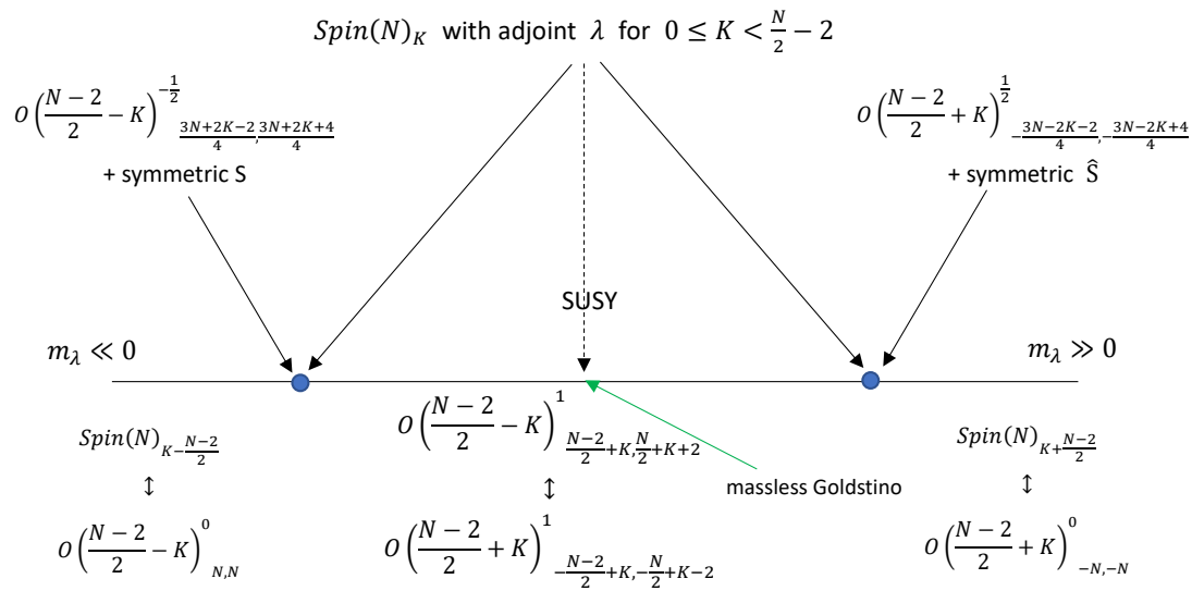
Figure 2: The phase diagram of Spin(N) gauge theory coupled to an adjoint fermion. The infrared TQFTs, together with relevant level-rank duals are shown along the bottom. The blue dots indicate transitions from the semiclassical phase to a quantum phase. Each transition is weakly coupled in a dual theory, which covers part of the phase diagram. The dual theory has symmetric tensor fermions ( S and \hat{S} ). Across these transitions the superscript level of the TQFT jumps, i.e. O(N)^0 and O(N)^1 are exchanged. The fractional levels represent the effective contributions from the massless fermions. At a special value of the mass in the quantum phase, the ultraviolet theory is supersymmetric. This symmetry is spontaneously broken leading to a massless Goldstino [37]. This phase diagram is obtained from that of the SO(N) theory proposed in [6], by tracking the global symmetries and counterterms and then gauging.
