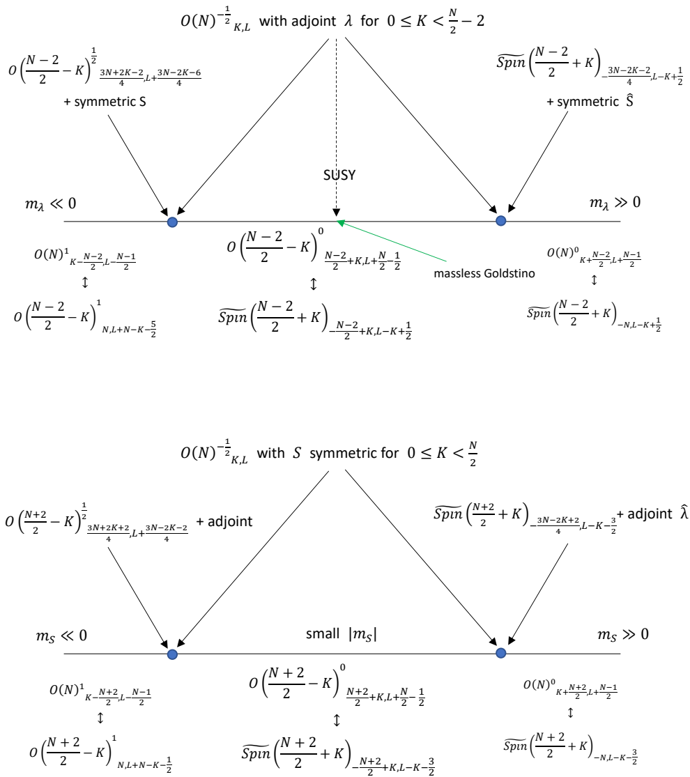
Figure 7: The phase diagrams of O(N)^{-\frac{1}{2}} gauge theory coupled tensor fermions. The infrared TQFTs, together with relevant level-rank duals are shown along the bottom. The blue dots indicate the transitions from the semiclassical phase to the quantum phase. This proceeds through a tensor transition described by a dual theory, which covers part of the phase diagram. Across these tensor transitions O(L)^0 and O(L)^1 are exchanged. At a special value of the mass in the quantum phase of the adjoint theory, a massless goldstino appears. The notation \widetilde{Spin}(N)_{K,L} is explained around (4.34).
