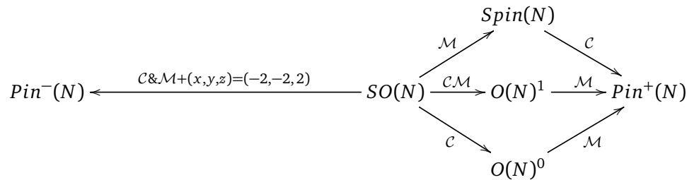
Figure 3: A map of possible gauge groups obtained by starting with SO(N) and gauging symmetries ( \mathbb{Z}_2 levels suppressed). In Appendix C we discuss some details of this map.
