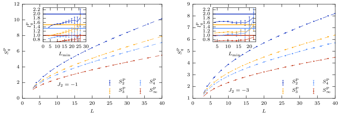
Figure 4: Participation entropies S_q^P of the line shaped subsystem A for J_2 = -1 (left) and J_2 = -3 (right) as a function of the linear system size L . The dashed lines display our best fits over the range L \in [10, 40] . The logarithmic term is visible and the inset shows the result of a fit to the form Eq. (9) over the fit range [L_{\min}, 40] as a function of L_{\min} . Horizontal lines are guides to the eye for q/(q-1) for q = 2, 3, 4 and q = \infty .
