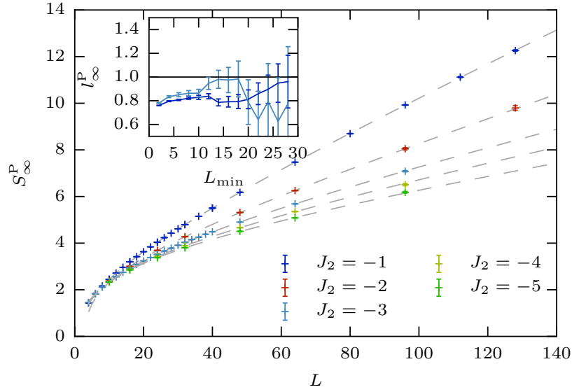
Figure 2: Participation entropy S_\infty^P of the line shaped subsystem for the T = 0 two-dimensional (panel (a) of Fig. 1) S = 1/2 Heisenberg model [Eq. (2)] at different values of J_2 . The inset shows the prefactor of the logarithmic term obtained from fits to the form Eq. (8), using different fit windows [L_{\min}, L_{\max}] as a function of L_{\min} for the two values of J_2 = -1 and J_2 = -3 , for which we have collected data on the finest grid in system size. L_{\max} is the maximal linear system size, ranging from 96 to 128. Our results are consistent with a universal logarithmic term with l_\infty = n_{\text{NG}}/2 = 1 , since for fit windows that include only large system sizes, the obtained l_\infty is close to 1 within errorbars.
