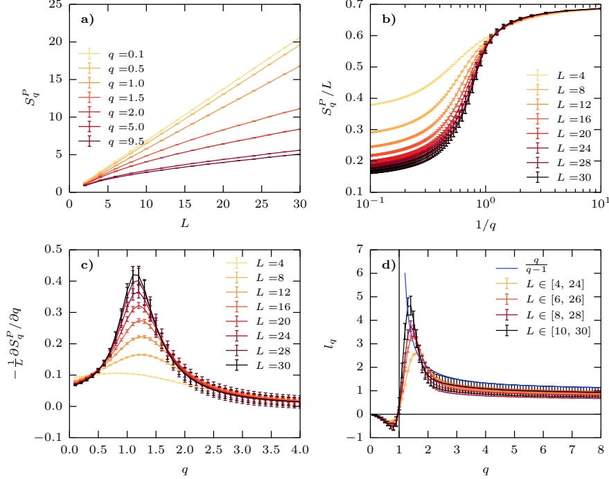
Figure 5: QMC results for the groundstate participation entropies S_q^P of a periodic line embedded in the L \times L two-dimensional J_1 - J_2 Hamiltonian Eq. (2) at J_1 = 1, J_2 = -1 , computed directly from the histogram of sampled basis states. (a) Entropies as a function of the linear system size L for some representative values of the Rényi parameter q . (b) Intensive part S_q^P/L plotted against 1/q for varying lengths L . An inflection point is demonstrated in panel (c) where the derivative is peaked around q_c \simeq 1 . (d) q -dependence of the prefactor l_q of the logarithmic correction obtained from fits to the form Eq. (11) performed over various windows, as indicated on the plot. The analytic prediction Eq. (10) is also shown for q > 1 (blue line). Panels (c-d) clearly show a Rényi index transition at q_c \simeq 1 .
