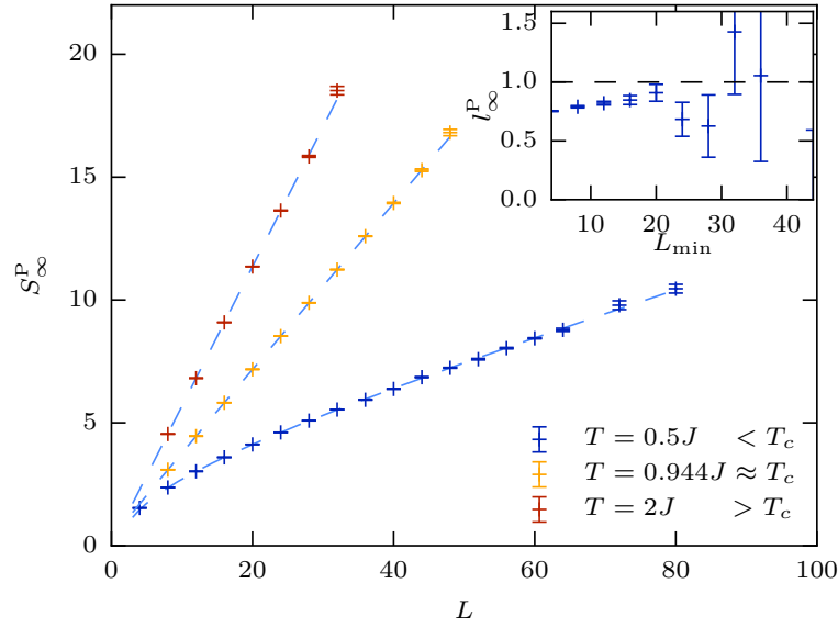
Figure 3: Participation entropy S_\infty^P of the line shaped subsystem in a three dimensional antiferromagnet (panel (b) of Fig. 1) at different temperatures. Below the critical temperature T_c , the thermodynamic limit ordering with a breaking of the continuous SU(2) symmetry shows up on finite systems as the participation entropy acquires a logarithmic correction term. The inset shows the prefactor of this logarithmic term obtained from fits to the form S_\infty^P = a_\infty L + l_\infty \ln L + b_\infty , which agrees well with l_\infty = 1 .
