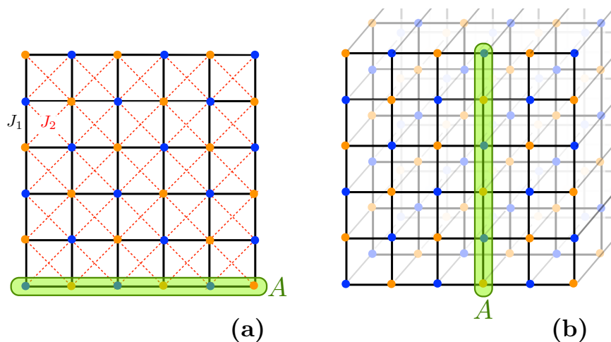
Figure 1: Schematic picture for the two lattice antiferromagnets. (a) The J_1 - J_2 Hamiltonian defined on a two-dimensional square lattice Eq. (2). (b) The nearest-neighbor Heisenberg model Eq. (3) on a three-dimensional cubic lattice. In both cases, the line shaped subsystem A is shown in green.
