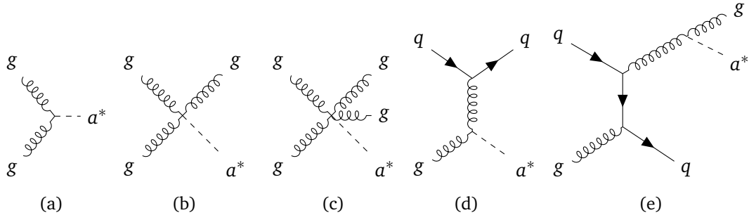
Figure 1: Some representative Feynman diagrams for the dominant ALP production mechanisms mediated by the QCD interaction at the LHC. Off-shell ALPs are produced through VBF, t -channel gluon exchange, ALPstrahlung, and variants thereof. Only diagrams with independent initial and final states are shown. Additional t -channel and ALPstrahlung topologies arise when considering different internal propagators.
