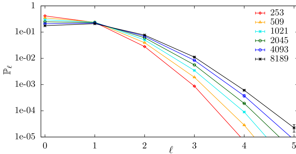
Figure 13: Probability distribution \mathbb{P}_\ell versus the nested-path number \ell for a series of sizes L for STc at criticality.
