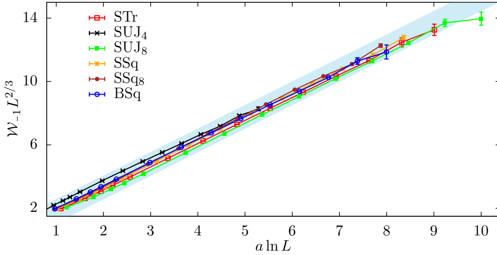
Figure 11: Illustration of the logarithmic correction by plotting \mathcal{W}_{-1} L^{2/3} versus a \ln L , with a a model-dependent constant (we set a = 1 for STr). The approximate linearity for all systems supports \mathcal{W}_{-1} \sim L^{-2/3}(\ln L) .
