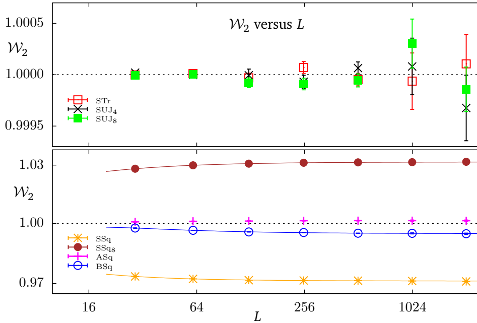
Figure 8: Plot of \mathcal{W}_2 versus the linear size L for STTr, SUJ 4 and SUJ 8 (top) and for BSq, SSq and SSq 8 (bottom). Also shown are the averaged data for SSq and SSq 8 , denoted by “ASq”. For triangulation lattices (top), the value of \mathcal{W}_2(L) is exactly 1 for any L , while for other lattices, \mathcal{W}_2(L \rightarrow \infty) converges to some constant slightly away from 1. The curves, obtained from the least-squares fits, are guides to the eye.
