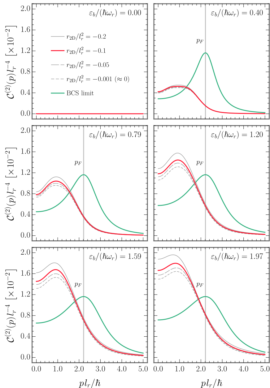
Figure 4: The calculated opposite-momentum pair correlator \mathcal{C}^{(2)}(p) as a function of momentum p for the ground state of N_\uparrow + N_\downarrow = 3 + 3 fermions. The multiple panels are associated with different interaction strengths \sim \varepsilon_b , whereas the axial confinement \sim r_{2D} is varied within each panel. In the experiment of Ref. [24] the measured binding energies were \varepsilon_b/(\hbar\omega_r) = 0.00, 0.79, 1.20 , and 1.97 , while the trap aspect ratio corresponded to an effective range of r_{2D}/l_r^2 = -0.1 (marked by the thick red line). The vertical gray line designates the Fermi momentum p_F .
