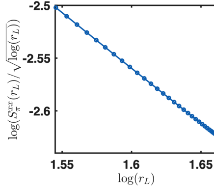
Figure 13: S_{\pi}^{xx}(r_L)/\ln^{1/2}(r_L) as function of r_L on a log-log scale where the slope is -1.043 , in which r_L = \frac{L}{\pi} \sin(\frac{\pi r}{L}) . DMRG numerics are performed for the gamma-staggered-octupole model in the U_6 frame on a system of L = 144 sites using periodic boundary conditions. The parameters are chosen as \Gamma = -1 , \Omega_2 = 0.3 .
