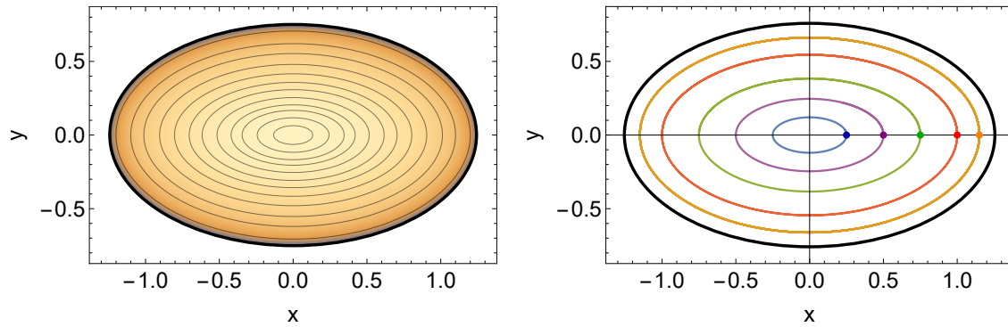
Figure 5: Left: constant-energy contours for a vortex inside an ellipse with aspect ratio b/a = 0.6 . The thick black line denotes the outer boundary with a = 5/4 and b = 3/4 . The vortex energy is negative and it decreases moving from the centre towards the boundary. Right: trajectories of a single vortex inside the same elliptical boundary for various initial positions on the positive horizontal axis. Coloured dots denote the starting point of the different trajectories, which are obtained from numerical solution of the equations of motion (43).
