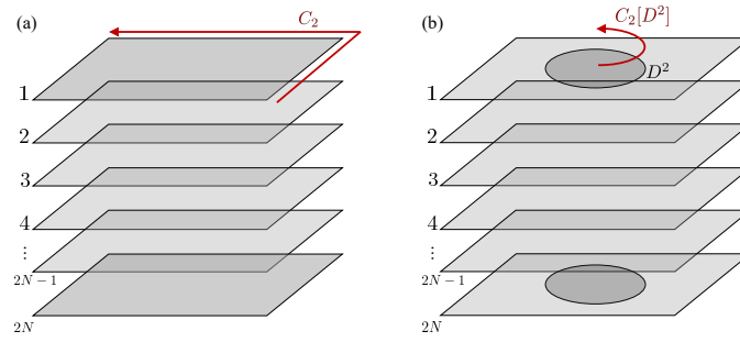
Figure 5: Boundary conditions of the layered system. (a): Twisted boundary condition for C_2 rotation symmetry acting on the whole 2d torus, which makes the topology of T^2 \rtimes_{C_2} S^1 . (b): Twisted boundary condition for the partial C_2 rotation acting on the disk within the 2d torus, which makes the topology of \mathbb{R}P^3 \# T^3 .
