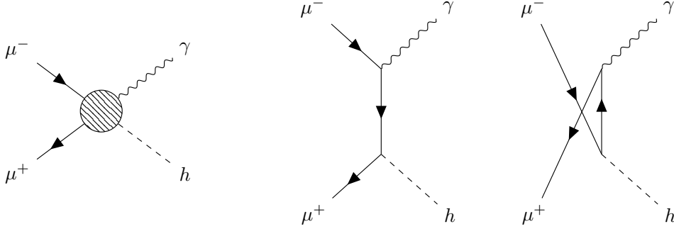
Figure 2: Contributions to \mu^+\mu^- \rightarrow \gamma h from SMEFT operators (left) and the Standard Model (right).
