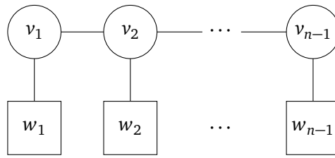
Figure 10: Quiver for the 3d \mathcal{N} = 4 theory T_{\varrho}[\mathrm{U}(N)]_K^L with N = \sum_{i=1}^n K_i = \sum_{j=1}^p L_j . The ranks of the gauge and flavor groups are defined form K and L via (4.86). \varrho = (\varrho_1^{\mathbb{C}}, \dots, \varrho_{p-1}^{\mathbb{C}}) where \hbar \varrho_j^{\mathbb{C}} s are complex twisted masses for the flavor symmetry. The mirror of this theory is denoted by T_{\varrho}^{\vee}[\mathrm{U}(N)]_K^L , if this also admits a quiver description then the quiver is given by Fig. 3.
