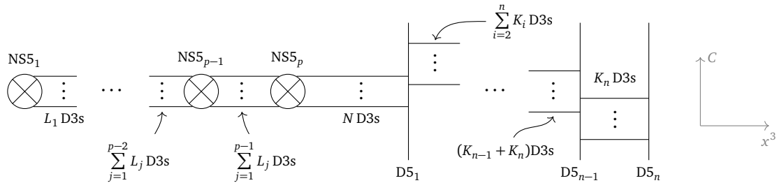
Figure 1: Brane configuration for the line operator \mathbb{L}_\rho(\mathbf{K}, \mathbf{L}) in \text{GL}_n 4d CS theory labeled by linking numbers \mathbf{K} = (K_1, \dots, K_n) and \mathbf{L} = (L_1, \dots, L_p) satisfying \sum_{i=1}^n K_i = \sum_{j=1}^p L_j = N . \hbar \varrho = \hbar(\varrho_1^C, \dots, \varrho_{p-1}^C) are complex FI parameters, they are not visible in the classical brane picture. We denote the 3d \mathcal{N} = 4 theory describing the low energy dynamics of the D3 branes by T_\varrho^\vee[\text{U}(N)]_K^L .
