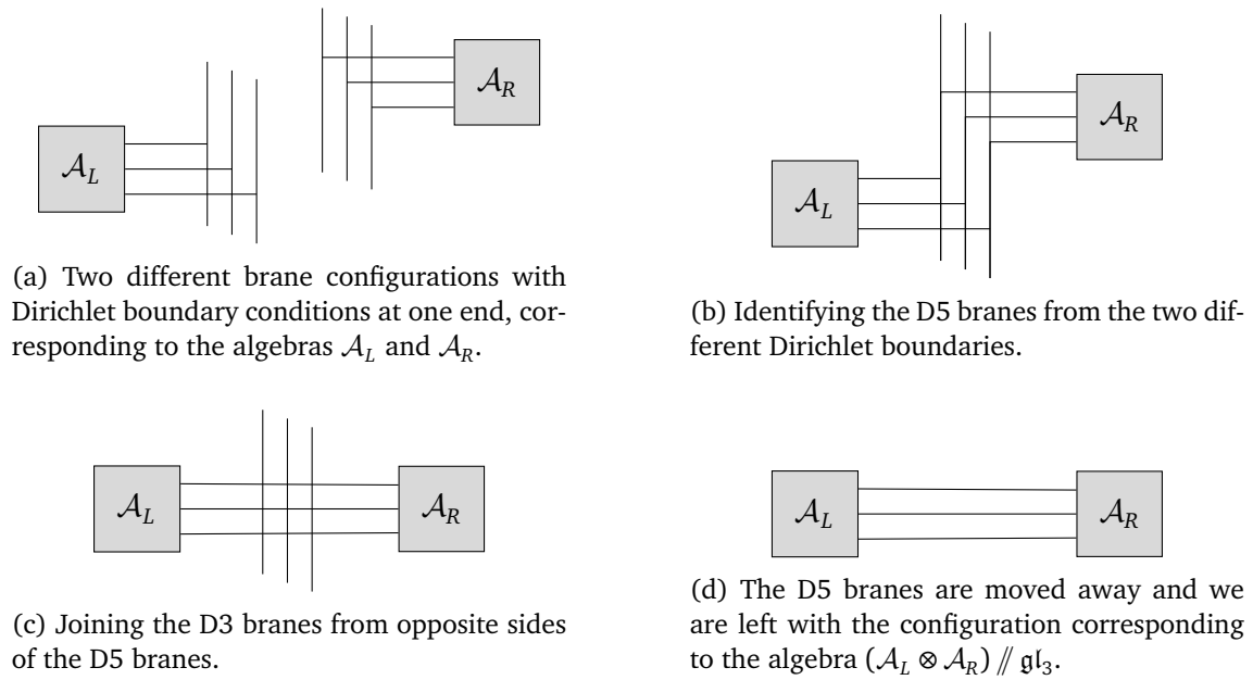
Figure 17: Gluing two boundary algebras \mathcal{A}_L and \mathcal{A}_R with Hamiltonian \mathrm{GL}_3 actions – the brane picture. The gray squares with \mathcal{A}_L and \mathcal{A}_R hide whatever configurations of branes are needed to get the algebras \mathcal{A}_L and \mathcal{A}_R . The vertical and horizontal lines are D5 and D3 branes respectively.
