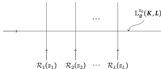
Figure 11: Schematic diagram of a \mathfrak{gl}_n spin chain with Hilbert space \mathcal{H} = \bigotimes_{i=1}^L \mathcal{R}_i(z_i) , realized in 4d \mathrm{GL}_n CS theory as an arrangement of vertical Wilson lines. \mathbb{L}_{\varrho}^{z_0}(K, L) has been introduced as a horizontal line operator to create the monodromy matrix \mathcal{L}_{\varrho}^{z_0}(K, L|\mathcal{H}) .
