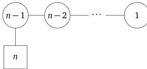
Figure 12: The quiver for the 3d \mathcal{N} = 4 theory T_{\varrho}[U(n)] , whose Coulomb branch is the phase space for the T-operator.
