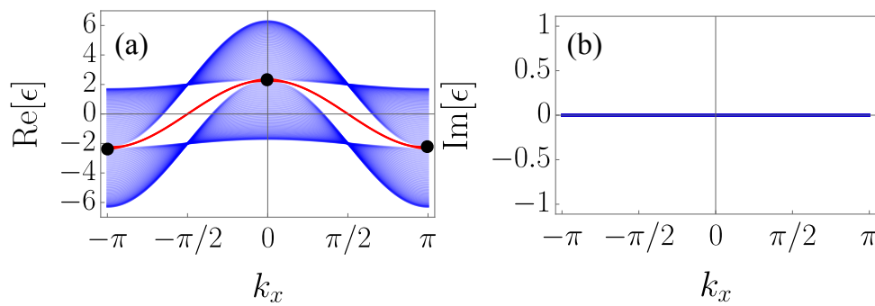
Figure 7: Real (a) and imaginary (b) part of spectra for Eq. (D.1) with open boundary condition in the y direction and at k_z = 0 . Red lines present boundary states. Black points mark ONPs. Here we set t = V = 1.0 , \lambda_0 = 2.3 .
