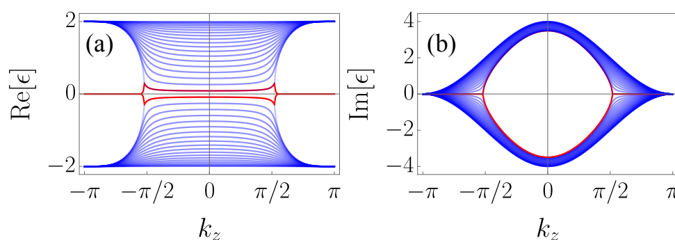
Figure 6: Real (a) and imaginary (b) part of spectra for Eq. (12) with open boundary condition in the y direction and k_x = 0 . Red lines present boundary states. Here we set t = V = \lambda_0 = 1.0 .
