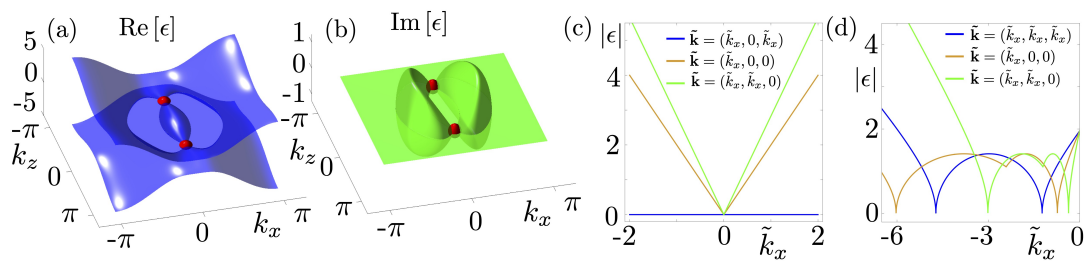
Figure 4: Real (a) and imaginary (b) part of band structure for \mathcal{H}_{\text{psH}}^{4b} in Eq. (19) along k_x = k_y and k_z . Note that along this particular cut, both bands are doubly degenerate. Red points indicate non-defective EPs at \mathbf{k} = (0, 0, \pm k_0) . Also here, it is clear that the absolute value of the eigenvalues depend linearly on the momentum components close to the non-defective EP at \mathbf{k} = (0, 0, k_0) [panel (c)], while a fractional behavior is observed around defective EPs, exemplified around \mathbf{k} = [\pi/2, \pi/2, \arccos(2 - \sqrt{2})] in panel (d). Here we set t = t_z = \lambda_{Ixx} = \lambda_{Ixy} = 1 , m'_I = -0.27 and k_0 = \pi/2 .
