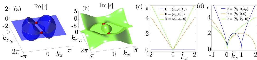
Figure 3: Real (a) and imaginary (b) part of band structure for \mathcal{H}_{\mathcal{PT}}^{2b} in Eq. (12) at k_y = 0 along k_x and k_z . Red points indicate non-defective EPs at \mathbf{k} = (0, 0, \pm k_0) . Panel (c) displays the linear dependence on the momentum of the absolute value of the eigenvalues at the non-defective EP \mathbf{k} = (0, 0, \pi/2) in different cuts of momentum space. We notice flat directions along the defective EP. To contrast this, panel (d) shows the fractional behavior of the absolute value of the eigenvalues around the defective EP at \mathbf{k} = (\pi/2, 0, \pi/2) in the same cuts. Here we set t = V = 1 , and \lambda_0 = 0 .
