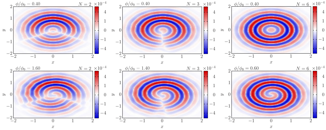
Figure 7: The interference G_{RC} between ring and center for N_p = 6 particles with N = 2, 3, 6 , as a function of the effective magnetic flux \phi at U = 1 and short time t = 0.025 . In the top panel, the number of dislocations in the interferograms is 2, 1, 0 for N = 2 (left), N = 3 (middle) and N = 6 (right) respectively. The bottom panel depicts the value of \phi where a spiral is observed. On increasing N , the spiral appears at a lower value of \phi since the displacement of the Fermi sphere is inversely proportional to N . All correlators are evaluated with DMRG for L = 15 by setting \mathbf{r}' = (0, R) and radius R = 1 . The color bar is non-linear by setting \text{sgn}(G_{RC})\sqrt{|G_{RC}|} .
