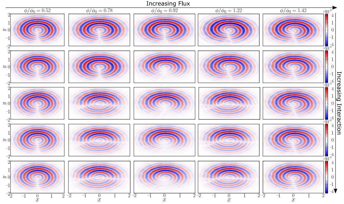
Figure 9: The interference G_{R,C} between ring and center for N_p = 4 particles with SU(2) symmetry against the effective magnetic flux \phi at short time t = 0.026 as a function of the interaction U . In this figure, one can clearly see how the number and orientation of the dislocations change as one increases the interaction. All correlators are evaluated with exact diagonalization for L = 15 and repulsive U = \{0, 10, 20, 50, 5000\} (panels are in descending order) by setting \mathbf{r}' = (0, R) and radius R = 1 . The color bar is non-linear by setting \text{sgn}(G_{R,C})\sqrt{|G_{R,C}|} .
