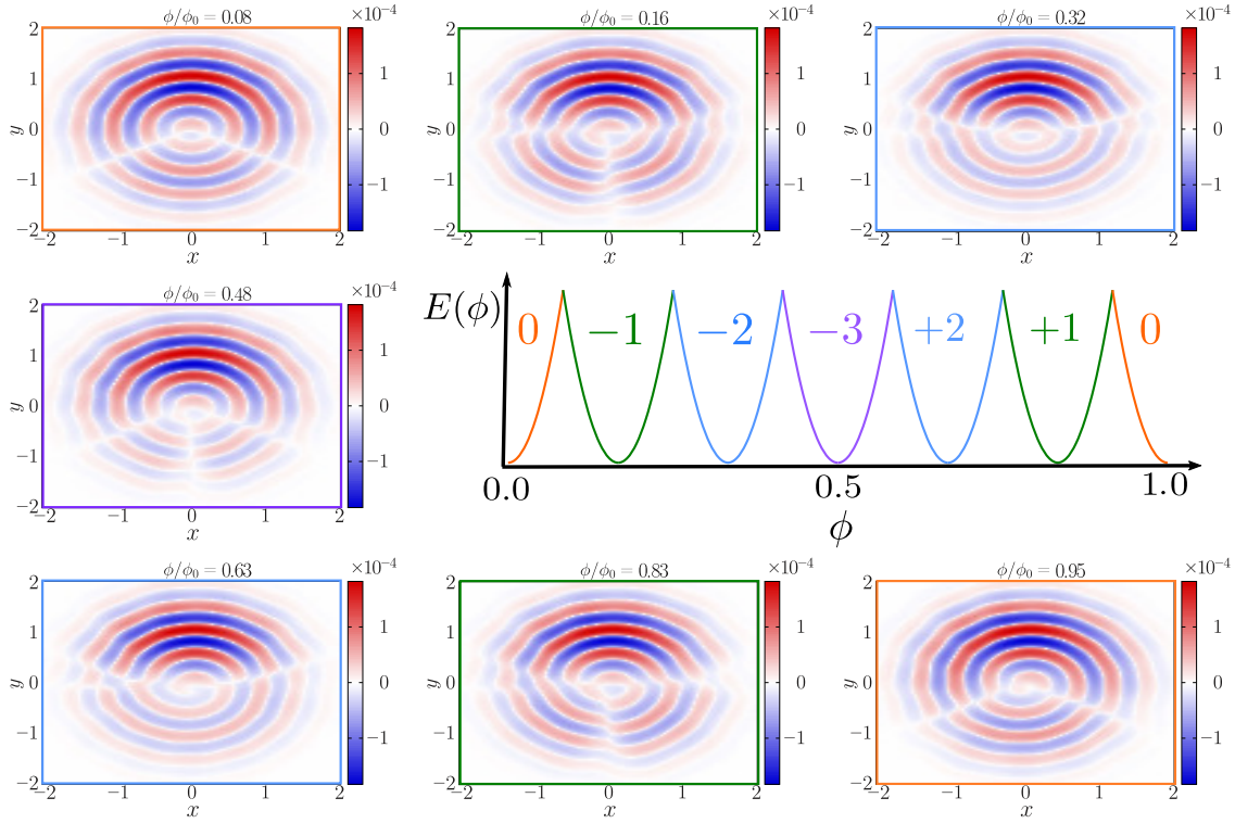
Figure 8: The interference G_{RC} between ring and center for N_p = 6 particles with SU(2) symmetry against the effective magnetic flux \phi at U = 1000 and short time t = 0.025 . Middle right panel is the schematic for the fractionalized energy parabolas at infinite repulsive interactions for the corresponding system (numbers on parabola correspond to the spin quantum numbers in the Bethe Ansatz solution [43]). The interference pattern corresponding to the first parabola (orange), displays two dislocations as in the zero interaction case. Moving to the next parabola (green), where we have the generation of a spin excitation, there are three dislocations. Traversing the other parabolas, we observe that apart from the number of dislocations, the orientation changes as well –see upper left and right panels where we observe an downward and upward V-shape respectively. By comparing each interference pattern to each energy parabola, we see that there is a symmetry around \phi = 0.5 that reflects the fact the the energy E is symmetric around this point. Indeed, the number of different interference patterns corresponds to \lceil \frac{N_p}{2} \rceil + 1 . Note that there is no spiral in the bottom right intereferogram since no hole has opened up. All correlators are evaluated with exact diagonalization for L = 15 by setting \mathbf{r}' = (0, R) and radius R = 1 . The color bar is non-linear by setting \text{sgn}(G_{RC})\sqrt{|G_{RC}|} .
