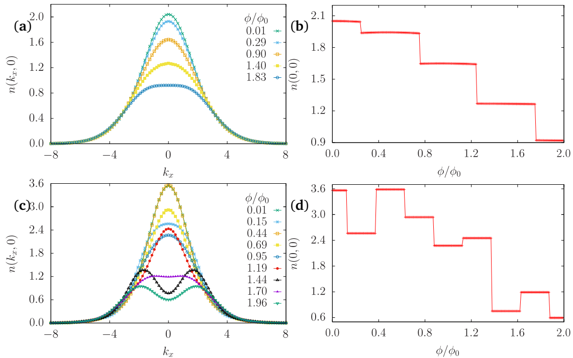
Figure 14: Left panel: Cross-section of the momentum distribution n(k_x, 0) for U = -5 (top) and U = 10,000 (bottom) as a function of the effective magnetic flux \phi . On the right panels, there is the corresponding momentum distribution n(0, 0) for k_x = k_y = 0 . Results were obtained with exact diagonalization for N_p = 4 , N = 2 for L = 15 .
