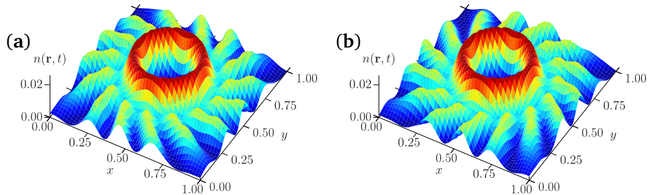
Figure 16: Density distribution n(\mathbf{r}, t) at an intermediate time t = 3 evaluated at \phi/\phi_0 = 4 and \phi/\phi_0 = -4 . The right (left) panel corresponds to \phi = 4 ( \phi = -4 ) and the direction of the protruding spirals is clockwise (anti-clockwise). The direction of the rotation by the artificial gauge field is reflected in the quantum shuriken. The results were calculated with exact diagonalization for N_p = 3 with N = 3 and L = 15 at U = 0 .
