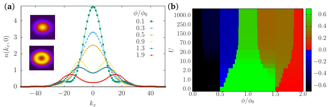
Figure 3: (a) Cross-section of the momentum distribution n(k_x, 0) at strong repulsive interactions U = 10,000 for various values of the effective magnetic flux \phi . When the threshold imposed by the fractionalization is surpassed, the momentum distribution collapses at k_x = 0 and a depression is observed. For larger values of \phi , the depth of the depression increases. (b) Second derivative of the momentum distribution n(k_x, k_y) evaluated at k_x = k_y = 0 , defined as \frac{\partial^2 n(k_x, 0)}{\partial k_x^2} \Big|_{k_x=0} , as a function of \phi and U . A change in the sign of the second derivative denotes going from a peak (negative) to a depression (positive) that corresponds to a change in colour from blue to green respectively. At U = 0 the hole opens up at \phi = 0.5 . On increasing the interaction, the depression appears at larger \phi thereby reflecting the fractionalization in the system. As U \rightarrow \infty , the system achieves complete fractionalization and the flux at which a depression is displayed corresponds to \phi_D . Note that the y-axis is not linear in values of the interaction. Results were obtained with exact diagonalization for N_p = 3 SU(3) symmetric in L = 15 sites.
