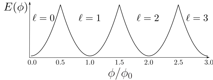
Figure 1: Energy as a function of the effective magnetic flux \phi , denoted by E and \phi respectively. As one crosses from one parabola to the next with increasing \phi , the angular momentum quantum number \ell increases.
