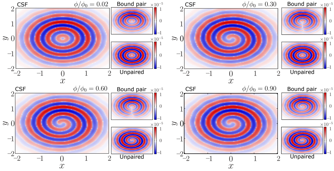
Figure 20: The interference G_{R,C} between ring and center for N_p = 3 three-component fermions in a CSF configuration, is shown as a function of the effective magnetic flux \phi at short time t = 0.0225 . Main panels corresponds to the CSF, upper panel to the two-body bound state and bottom panel to the unpaired particles. All correlators are evaluated with exact DMRG for L = 15 by setting \mathbf{r}' = (0, R) and radius R = 1 . The CSF configurations is achieved by |U_{AB}| = |U_{BC}| = 0.01 and |U_{AC}| = 3 . The color bar is non-linear by setting \text{sgn}(G_{R,C})|G_{R,C}|^{1/4} .
