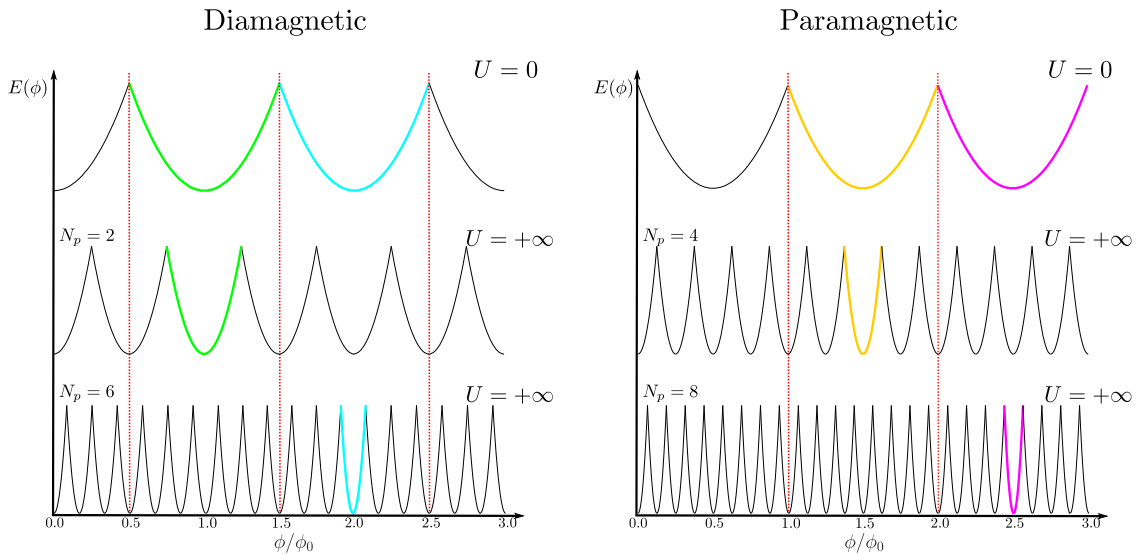
Figure 12: Schematic figure of the energy E against effective magnetic flux \phi for diamagnetic (left) and paramagnetic (right) cases. Top panel depicts the diamagnetic and paramagnetic cases at zero interaction for SU(2) fermions (holds for any N ). The middle panel shows the system for 2 and 4 particles with infinite repulsive interaction U . Comparing this panel with the one at U = 0 , we see that the hole for N_p = 2 (green) and N_p = 4 (yellow) is delayed on going to infinite repulsion. Likewise for N_p = 6 (cyan) and N_p = 8 (magenta), we also observe a delay in addition to the one that is observed at U = 0 (see Fig. (11)).
