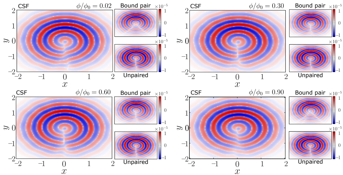
Figure 21: The interference G_{R,C} between ring and center for N_p = 6 three-component fermions in a CSF configuration, is shown as a function of the effective magnetic flux \phi at short time t = 0.0225 . Main panels corresponds to the CSF, upper panel to the two-body bound state and bottom panel to the unpaired particles. All correlators are evaluated with DMRG for L = 15 by setting \mathbf{r}' = (0, R) and radius R = 1 . The CSF configurations is achieved by |U_{AB}| = |U_{BC}| = 0.01 and |U_{AC}| = 3 . The color bar is non-linear by setting \text{sgn}(G_{R,C})|G_{R,C}|^{1/4} .
