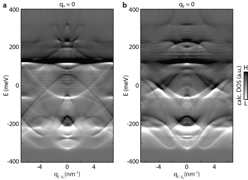
Figure 10: Calculated QPI using Green's function approach. a,b , Calculated QPI cut along \Gamma - X_1 and \Gamma - X_2 direction, respectively.
