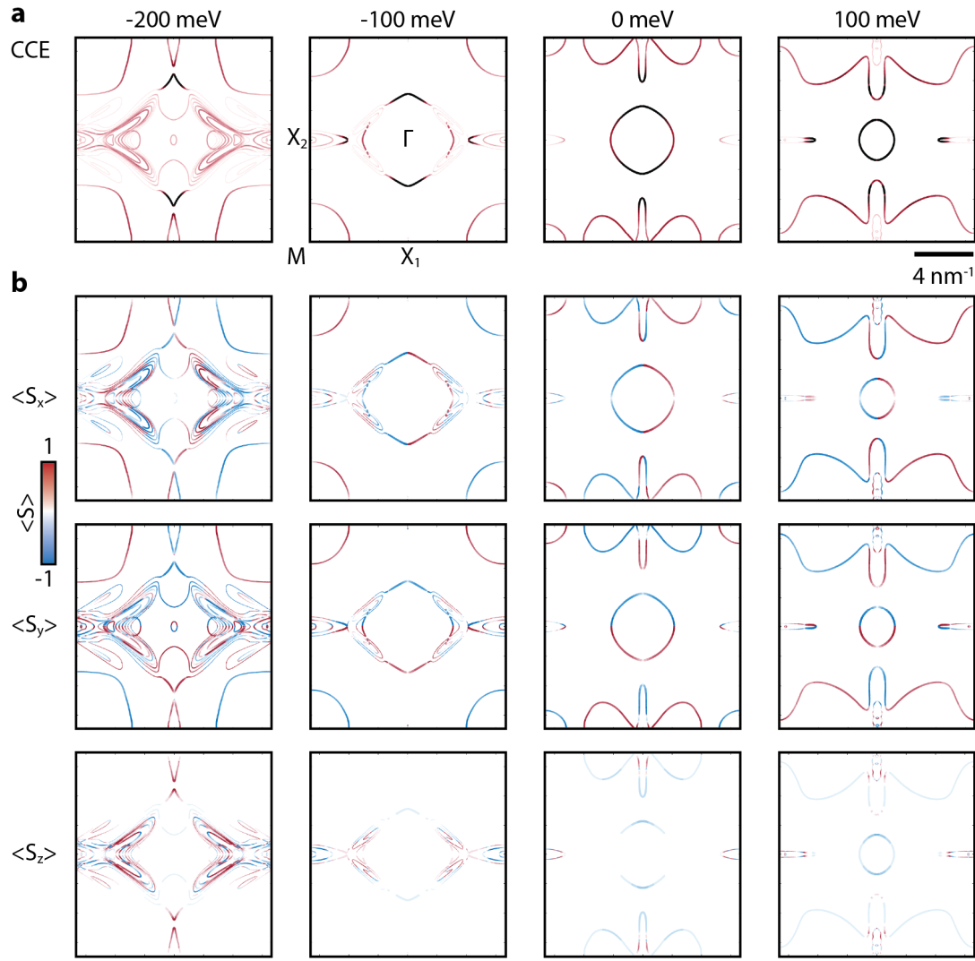
Figure 9: Calculated spin texture of the Bi(110) surface. a , CCEs of the Bi(110) band structure at representative energies. b , Normalized spin components of the corresponding CCEs in a .
