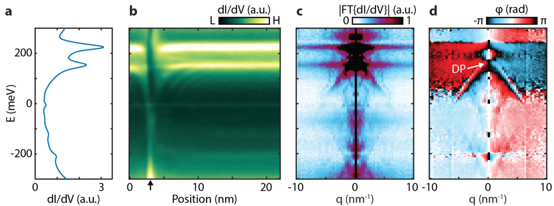
Figure 6: dI/dV map on Bi(110) sample #2. Similar measurement as Fig.5 for sample #2.
