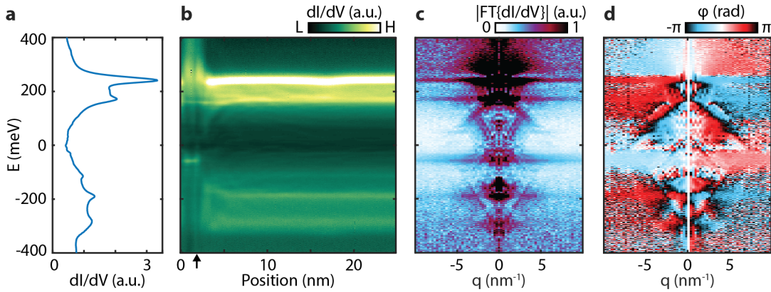
Figure 5: dI/dV map on Bi(110) sample #1. a , dI/dV profile measured far from the step edge. b , dI/dV mapping of the QPI patterns due to scattering off the step edge (marked by black arrow). c,d , The magnitude (same as Fig.3c) and the phase ( \phi ) of the Fourier transform of b showing the various dispersing modes, respectively.
