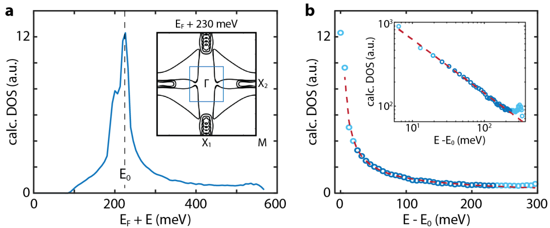
Figure 12: DFT calculated DOS on Bi(110). a , Momentum integrated DOS extracted from DFT surface band structure in the vicinity of the zone center (marked by blue box in inset). Inset: Contour of constant energy at 230 meV above the Fermi energy. b , Power-law fit to the calculated DOS, a(E - E_0)^b + c . The fit yields an exponent of b = 0.67(3) . Inset shows linear fit to log-log plot, m(E - E_0) + c . The fit yields a slope of m = 0.67(2) .
