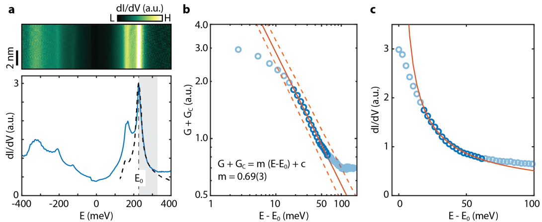
Figure 13: Diverging DOS on the Bi(110) surface. a , dI/dV map on Bi(110) away from defects (upper panel) and spatially averaged dI/dV profile overlaid with calculated DOS (lower panel). b-c , Log-log and linear plot of the dI/dV profile close to the diverging peak ( E_0 ) marked by the shaded region in a . Linear and corresponding power-law fit to the density of states is shown in b and c , respectively.
