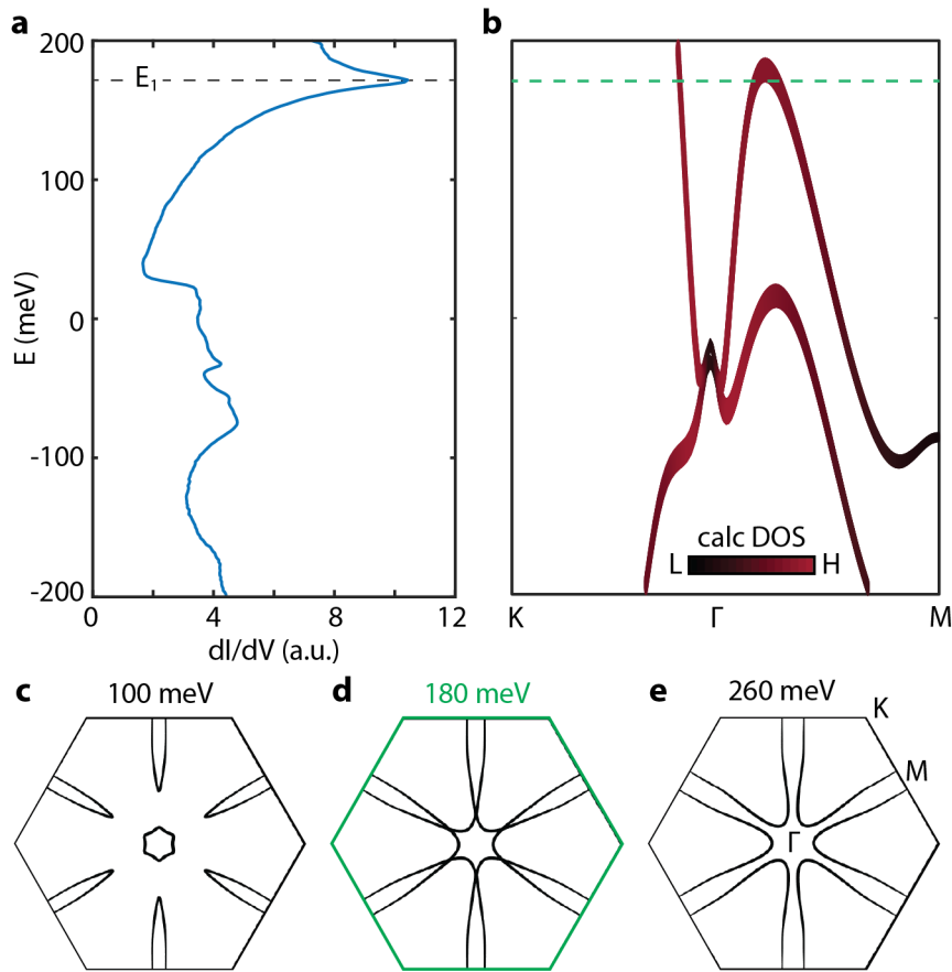
Figure 11: Calculated band structure of Bi(111) surface. a , A typical dI/dV profile measured on a clean (111) surface (same as Fig.2f). b , Ab initio calculated band structure of the Bi(111) surface along a high symmetry line. c-e , Contours of constant energy showing the evolution of the bands in the vicinity of the Lifshitz transition (green) responsible for the E_1 peak.
