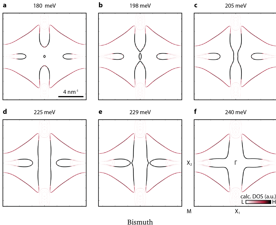
Figure 14: Calculated band structure of Bi(110) surface. Evolution of the Bi(110) surface band structure across Lifshitz transition in b and e . The nearly tangential band touching in e may give rise to high-order van Hove singularity.
