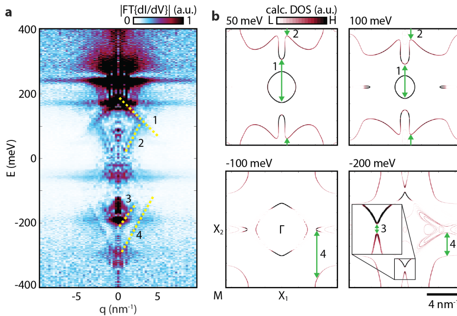
Figure 8: Various scattering wave vectors. a , Fourier transform of dI/dV measurement (same as Fig.3c). b , Scattering wave vectors are labeled and marked (green arrows) on some of the representative CCEs of the Bi(110) surface band structure.
