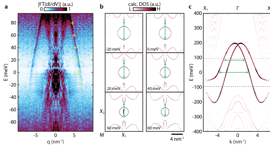
Figure 7: Scattering across Dirac bands. a , Fourier transform of the measured dI/dV profile on Bi(110) surface (same as Fig.1b). b , Calculated CCEs for the Bi(110) surface. The scattering process at various energies is marked by the green arrows. The corresponding q values are plotted in a as yellow '+'. c , Calculated band structure of Bi(110) surface along the high-symmetry direction X_1 - \Gamma - X_1 .
