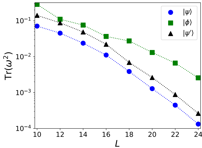
Figure 2: \text{Tr}[\omega^2] for a variety of system sizes and states. Numerics were done with the same model as Fig. 1, which is non-integrable. The three states studied are |\psi\rangle := |\uparrow\downarrow\uparrow\downarrow \dots\rangle , |\psi'\rangle := \frac{1}{\sqrt{2}}(|\uparrow\downarrow\uparrow\downarrow \dots\rangle + |\downarrow\uparrow\downarrow\uparrow \dots\rangle) and |\phi\rangle := \frac{1}{\sqrt{L}} \sum_{r=0}^{L-1} \hat{T}^r |\uparrow\uparrow \dots \uparrow\downarrow \dots \downarrow\downarrow\rangle where \hat{T} is the translation operator shifting lattice indices by one. More details on the states and the model can be found in App. D.
