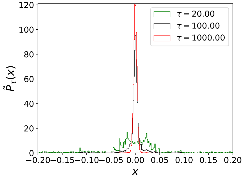
Figure 1: Convergence of P_T(x) to P(x) where P_T(x) = \int_0^T \frac{dt}{T} \delta(x - \langle A(t) \rangle) and P(x) is recovered as T \rightarrow \infty . \tilde{P}_T(x) represents the approximation of P_T(x) by binning samples and constructing a histogram. 1000 bins were used to create this histogram. Numerics were performed on a spin 1/2 chain with 22 sites. The data is normalized such that \int_{-\infty}^{\infty} \tilde{P}_T(x) dx = 1 . The Hamiltonian is a Heisenberg type model with nearest and next nearest neighbour interactions. The parameters in the Hamiltonian are chosen so that we have a non-integrable model. Further details can be found in App. D.
