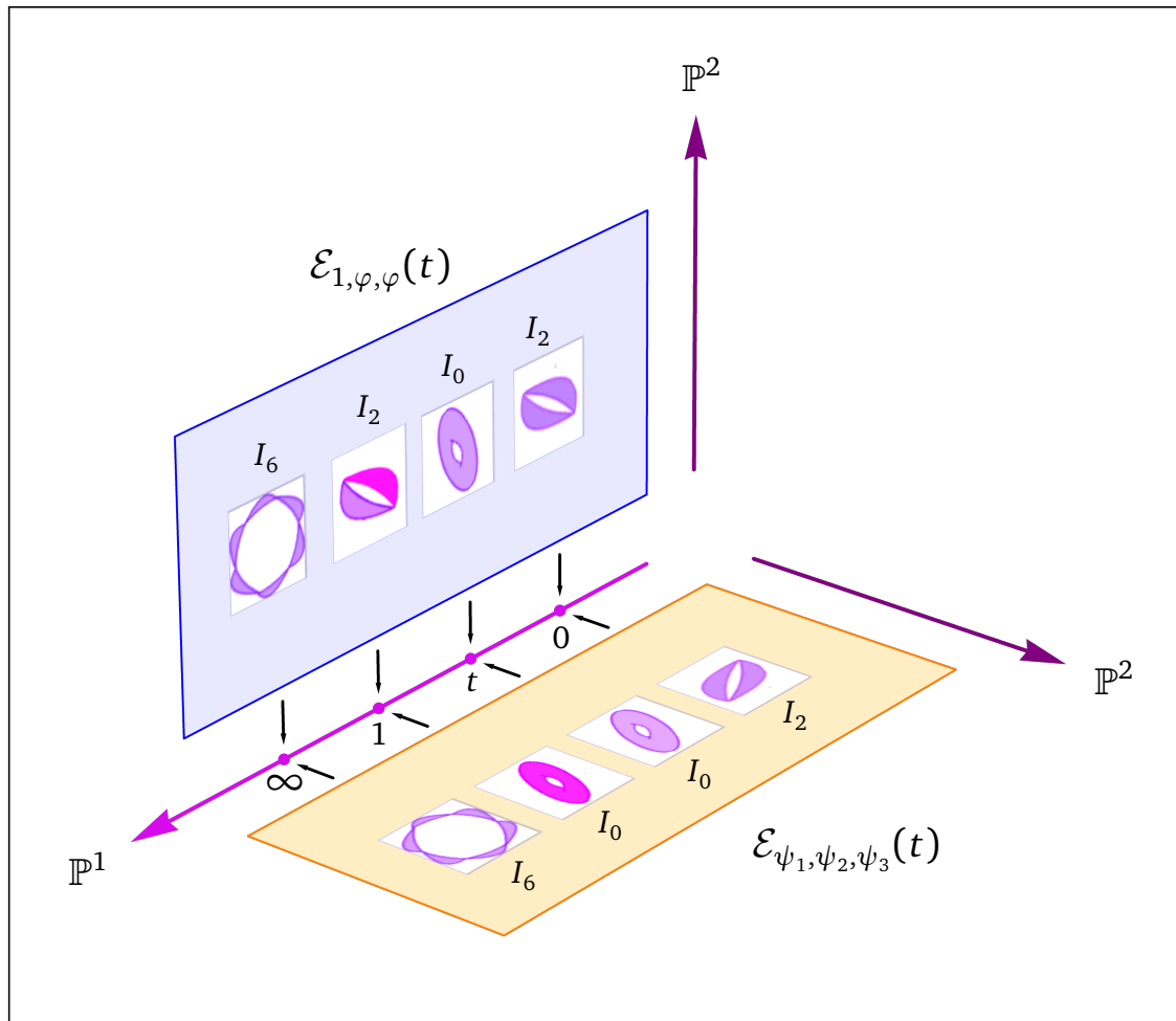
Figure 3: The \mathbb{Z}_2 symmetric Hulek-Verrill manifolds are birational to fibred products \mathcal{E}_{1,\varphi,\varphi}(t) \times_{\mathbb{P}^1} \mathcal{E}_{\psi_1,\psi_2,\psi_3}(t) over \mathbb{P}^1 with generic fibers elliptic curves \mathcal{E}_{\psi_1,\psi_2,\psi_3}(t) and \mathcal{E}_{1,\varphi,\varphi}(t) . In this sketch, this situation is depicted for generic values of \varphi, \psi_1, \psi_2 and \psi_3 . For generic t \in \mathbb{P}^1 the two elliptic curves are both smooth, however the fibers are singular for t = 0, 1, \infty , and certain other values. When t = 0 , both elliptic curves are singular curves of type I_2 ; when t = 1 one elliptic curve is smooth, while the other is of type I_2 ; and when t = \infty , both elliptic curves are singular of type I_6 . The remaining singular fibers over the points t_{\pm\pm} , which we do not display, contain I_1 singularities. The elliptic surface birational to the intersection \{X_1 + X_2 = 0\} \cap \text{HV}_\varphi \cap \mathbb{T}^5 consists of one of the distinct components of the singular fibre \mathcal{E}_{1,\varphi,\varphi}(t) , which is of type I_2 , together with the smooth elliptic curve \mathcal{E}_{\psi_1,\psi_2,\psi_3}(1) . This elliptic surface \mathcal{E}_{\psi_1,\psi_2,\psi_3}(1) \times \mathbb{P}^1 is highlighted in magenta.
