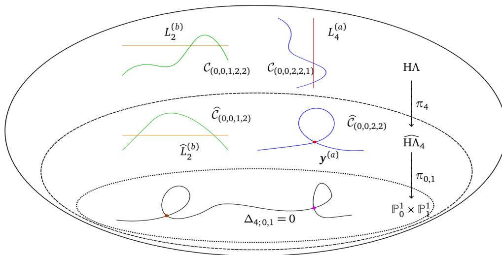
Figure 12: Schematic representation of elliptic fibres containing lines on HA . For concreteness, we have chosen here i = 4 , m = 0 , and n = 1 . The largest oval represents the smooth manifold HA , on which the elliptic fibration over \mathbb{P}_0 \times \mathbb{P}_1 contains unions of two rational curves. Here we have pictured the fibres which consist of one line and a degree-5 curve.
