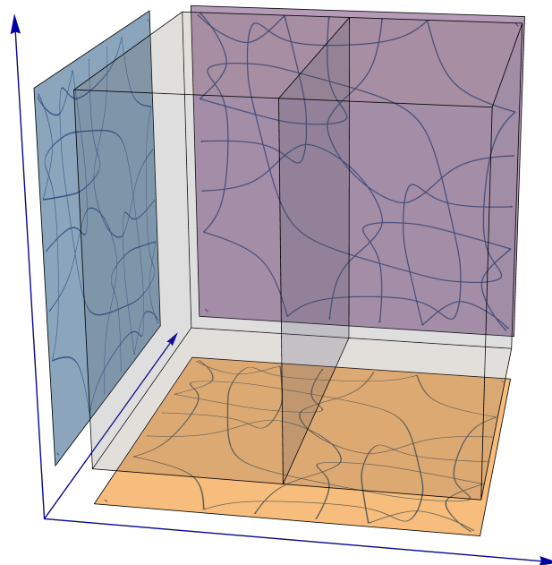
Figure 10: A heuristic sketch of the multiple fibrations. Each axis corresponds to a \mathbb{P}^1 , and the indicated plane corresponds to a K3 fibre of a projection to one of the \mathbb{P}^1 's.
