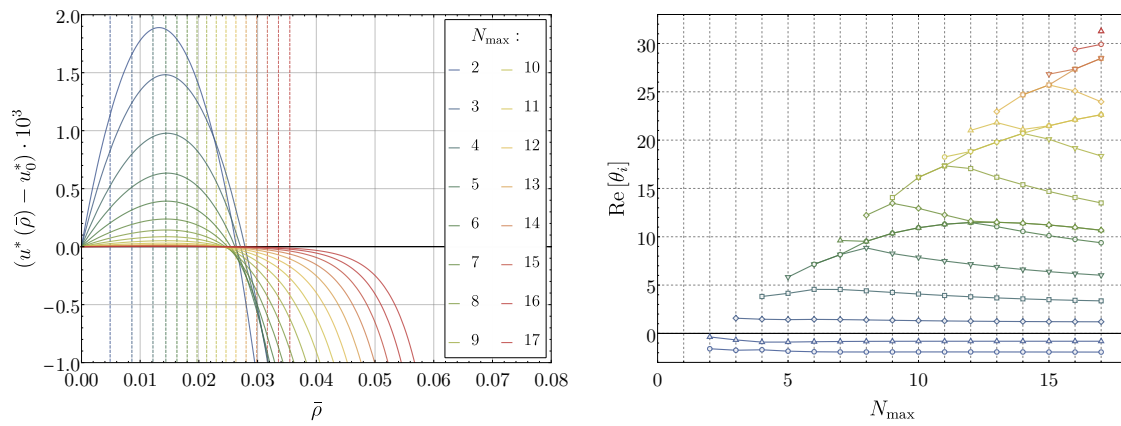
Figure 5: ASSM fixed point Higgs potential (left) and its critical exponents (right). The Higgs potential converges towards a flat potential within the reliability regime, which is indicated by the vertical lines as defined in (55). In contradistinction to a standard Gaussian Higgs potential with one relevant direction, we find two relevant directions related to the two negative eigenvalues (right) for all approximations, and the eigendirections have strong overlap with \lambda_{\Phi,2} (blue triangle) and \lambda_{\Phi,2N_{\max}} (blue circle), see Figure 6. The values rapidly converge with increasing N_{\max} , see (56). This rapid convergence is also seen for the lower lying positive eigenvalues, while the convergence of the large ones would require larger N_{\max} . The parameter space where such a non-trivial flat potential exist is indicated as the green regime in Figure 9, which includes the ASSM fixed point.
