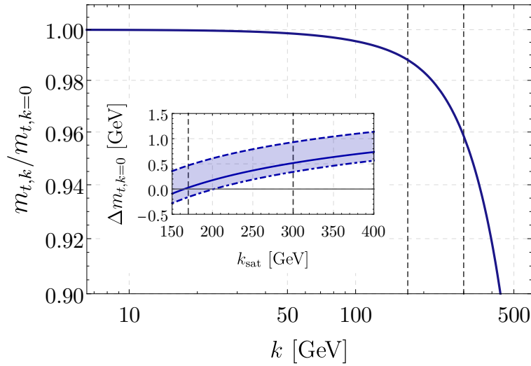
Figure 19: Top mass parameter m_{t,k} measured in units of m_t = m_{t,k=0} as a function of the cutoff scale. The mass parameter saturates at cutoff scales k \approx 200 GeV, and the vertical lines indicate the borders of the cutoff range (G.11) for k_{\text{sat}} . In the inlay, we depict the variation of m_t required for the experimental pole mass (45e) as a function of the saturation scale k_{\text{sat}} used for g_{3,k=k_{\text{sat}}} in (G.21). The upper dashed line is obtained for \alpha_s = \bar{\alpha}_s , the lower dot-dashed line is obtained for \alpha_s = 1.1 \bar{\alpha}_s (see (F.5)) and the central plain line for the ASSM flavour number extrapolation \alpha_s = 1.07 \bar{\alpha}_s . This covers the uncertainty in mapping the \overline{\text{MS}} -value of the coupling to the \text{MOM}^2 value used in the fRG computation.
