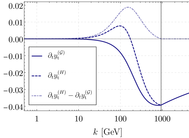
Figure 17: Flow of the top-quark Godstone (plain) and Higgs (dashed) Yukawa couplings defined in (F.7) and their difference (dot-dashed) (F.8). The difference is given by the scalar-field dependence of the Yukawa coupling. In the symmetric phase both couplings agree due to equal vanishing background.
