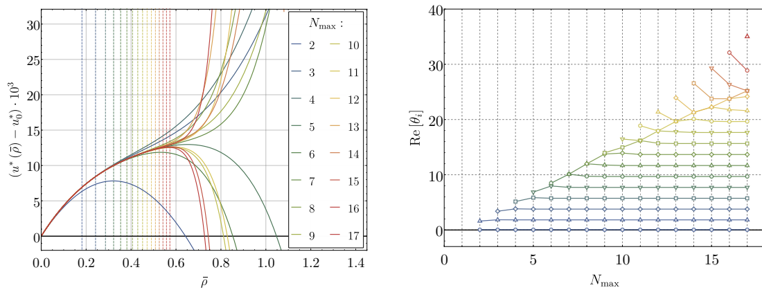
Figure 15: UV potential (left) and critical exponents (right) at different orders of the Taylor expansion for the gravitational fixed-point (B) in Figure 9 with g_h = 0.190 and \mu_h = -0.695 . The vertical dashed lines in the left panel show the reliability regimes at each order of the Taylor expansion with a relative error of 1% as defined in (55). The minimum critical exponent is \min[\theta_i^{(B)}] = 0.043 and therefore, the fixed point (B) has no relevant direction and shows a maximal predictivity. As discussed in Section 5.1, the IR trajectory of this FP does not lead to a physical IR.
