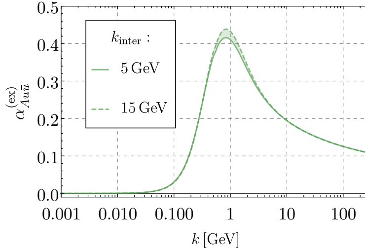
Figure 12: The quark-gluon exchange coupling \alpha_{Au\bar{u}}^{(ex)} defined in (C.21) as a function of k for interface scales k_{\text{inter}} = 5, 15 GeV. The chosen k_{\text{inter}} does not affect severely the IR dynamics.
