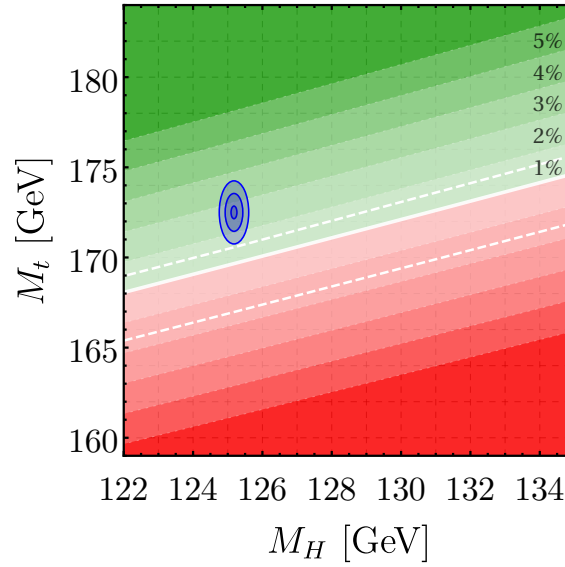
Figure 10: Values of M_H and M_t that can be reached from the non-trivial flat Higgs potential presented in Figure 5 (green region), that can be reached from the standard Gaußian fixed-point Higgs potential (white line), and that cannot be reached from either fixed point (red region). The white shadings show the 1%, ..., 5% error bands. The blue ellipsis displays the SM experimental measurement at 1\sigma , 3\sigma , and 5\sigma . The upper and lower dashed lines correspond to the Gaußian fixed-point trajectory for \alpha_{s,k=M_Z} = 1.1 \bar{\alpha}_s and \alpha_{s,k=M_Z} = \bar{\alpha}_s respectively.
