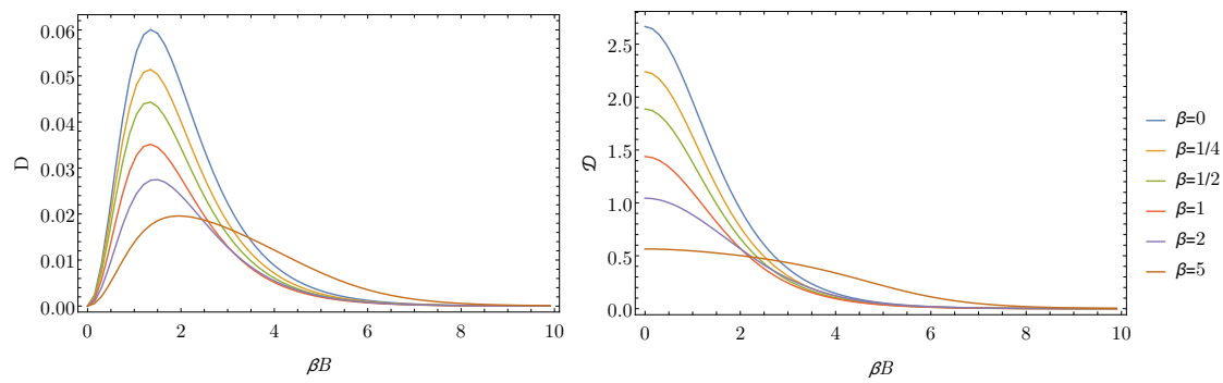
Figure 2: Magnetic field dependence of the Drude weight and the diffusion constant for various temperatures, h = 1 .
