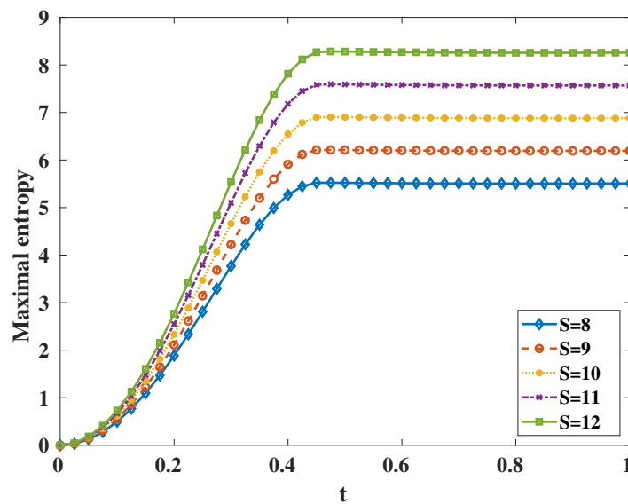
Figure 5: Maximum Rényi entropy ( \alpha = 2 ) as a function of t (time) averaged over 100 realizations of the unitary for different particle numbers S and fixed mode number M = 200 .
