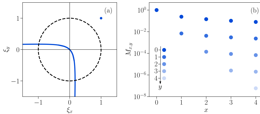
Figure 5: Exponentially localized charges at the corners. (a) Solutions of Eq. (17). The black dashed line shows the unit circle. (b) Largest value of Mazur's bound in Eq. (18) over the set of solutions plotted in panel (a), at different coordinates (x, y) .
