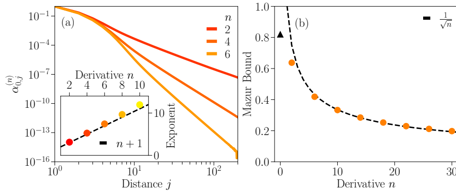
Figure 8: Mazur's bound and higher-moment distributions. (a) Power-law decay of higher-moment charges with modulation \alpha_{0,j}^{(n)} \sim j^{-(n+1)} as predicted from the continuum Laplace equation. (b) Dependence of Mazur's bound (15) with n , when including a single higher-moment charge with modulation \alpha^{(n)} . Mazur's bound including all n = 0 charges at the boundaries is shown as a black triangle. For this data we used a linear system size of L = 300 .
