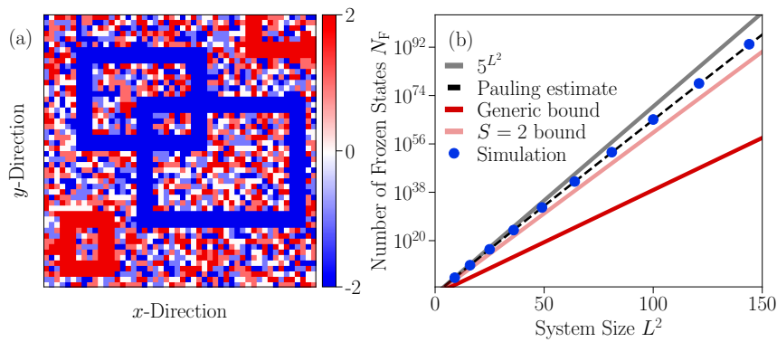
Figure 4: Fragmentation. (a): Construction of various sectors in configuration space using corollary 1, with inert walls splitting the lattice into disconnected regions. (b) Estimates for the number of completely frozen configurations, along with a Pauling estimate (see main text). Numerical simulations use system sizes with L \leq 12 .
