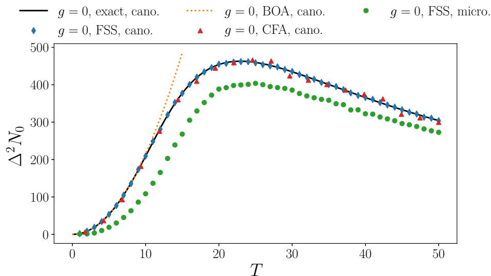
Figure 2: Fluctuations of a non-interacting Bose gas containing N = 100 atoms in a 1D ring trap. The variance of N_0 as a function of temperature in 1D in canonical ensemble is obtained from several different approaches: FSS method, classical field approximation, Bogoliubov approach (BOA) and an exact method (see text). In addition a microcanonical calculation using the FSS method is presented, showing the clear reduction of the expected fluctuations in this ensemble. The temperature T is given in units 2\pi^2\hbar^2/(mk_B L^2) .
