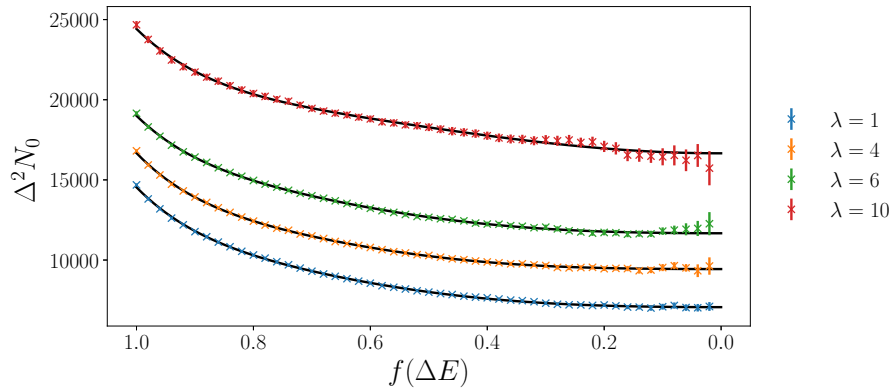
Figure 7: Fluctuations of atom number obtained after post-selection. The atom number variance \Delta^2 N_0 for different aspect ratios \lambda is shown as a function of the fraction f after post-selection. Thus the figure represents the transition from a canonical to a microcanonical result from left to right with solid black lines showing the polynomial fits. The initial sets represent N = 10^4 atoms at the temperature T_{\max} at which the canonical variance is maximal.
