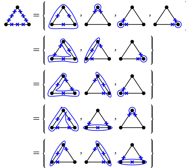
Figure 5: Higher codimension intersections of the facets outside \mathcal{P}_G . They can be graphically obtained by considering a set of k < n_s + n_e subgraphs which completely marks the graph \mathcal{G} in such a way that they do not share any marking.
