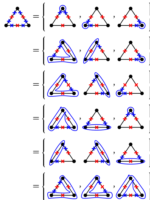
Figure 7: Higher codimension intersections of the facets outside \mathcal{S}_{\mathcal{G}} . They can be graphically obtained by considering a set of k < n_s + n_e subgraphs which completely marks the graph \mathcal{G} in such a way that they do not share any marking. The red marking \times , while the blue one \times indicates the one introduced by a subgraph. All but the last are in common with the cosmological polytope analysis — for the full cosmological polytope, the last set can appear in a triangulation through more than one subsets of the locus \mathcal{C}(\mathcal{P}_{\mathcal{G}}) .
