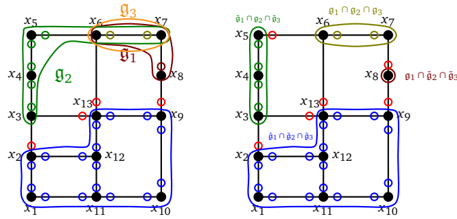
Figure 6: The intersection of the three facets identified by the subgraphs g_1 , g_2 and g_3 on the scattering facet \mathcal{S}_G [34].
