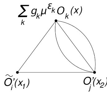
Figure 2: Linear order contribution to the correlator \langle \tilde{\mathcal{O}}'_i(x_1) \mathcal{O}'_j(x_2) \rangle . Solid lines represent propagators of the scalar fields. Integration is done over the insertion point x .
